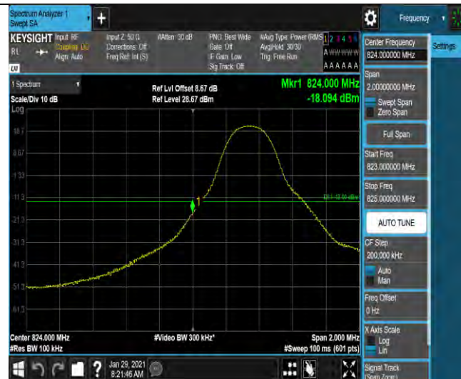
Band26-5MHz-QPSK-26815-1RB#24
