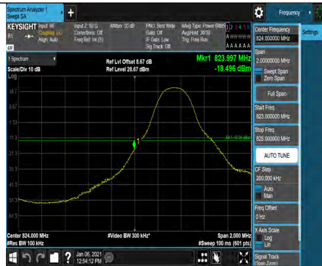
Band5-5MHz-QPSK-20425-1RB#24
