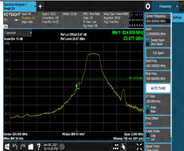
Band5-1.4MHz-QPSK-20407-1RB#5
