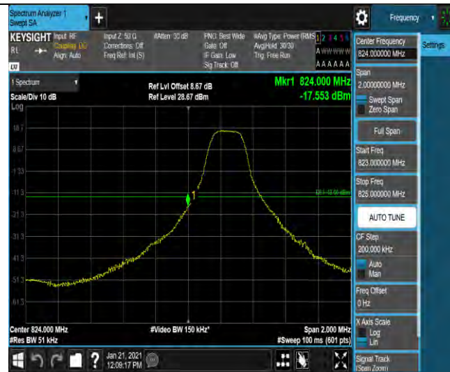
Band5-3MHz-16QAM-20415-1RB#14
