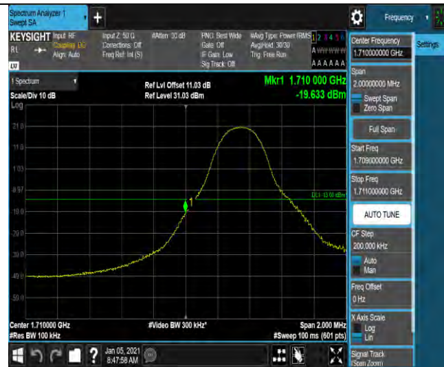
Band4-5MHz-16QAM-19975-1RB#24
