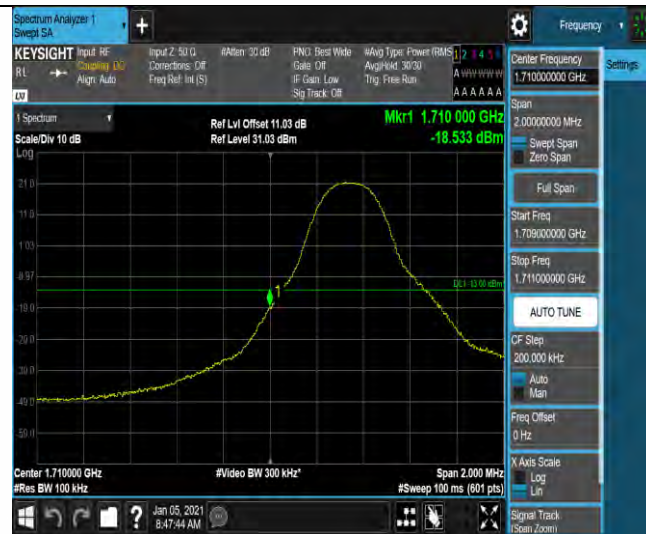
Band4-5MHz-QPSK-19975-1RB#24
