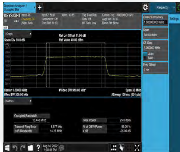
Band2-15MHz-16QAM-19125-75RB#0
