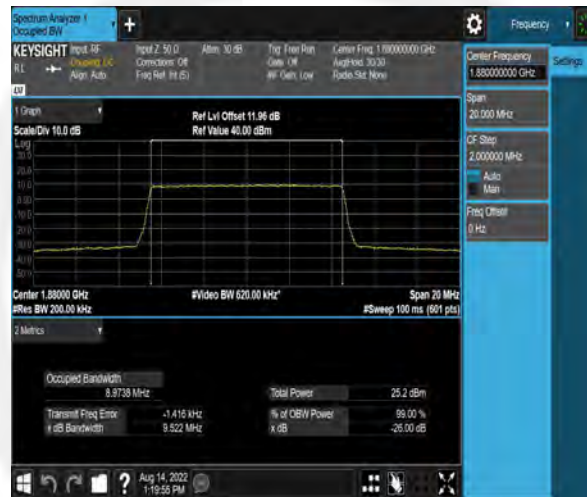
Band2-10MHz-16QAM-19150-50RB#0
