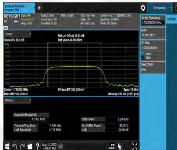
Band4-1413-4
