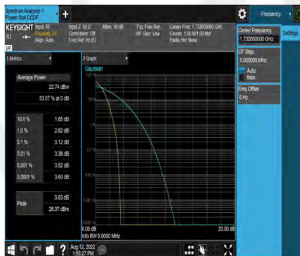
Band4-1513
