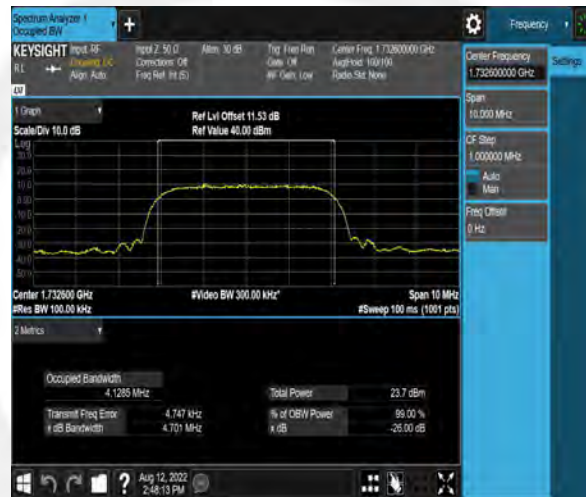
Band4-1513-1
