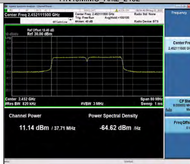
11N40MIMO Ant2 2452
