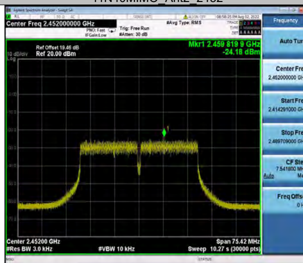
11N40MIMO Ant2 2452
