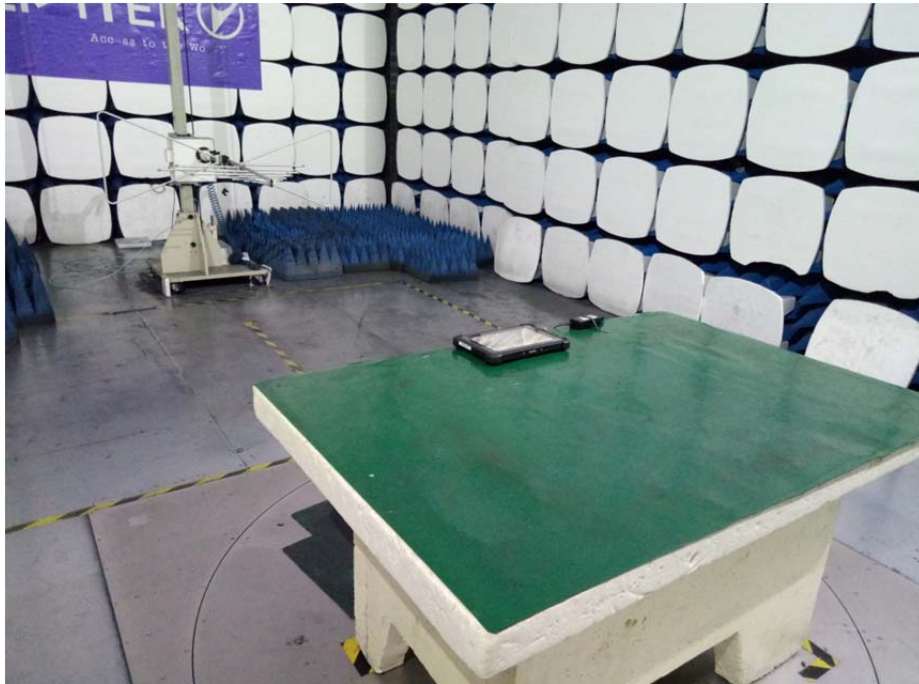
Test setup
