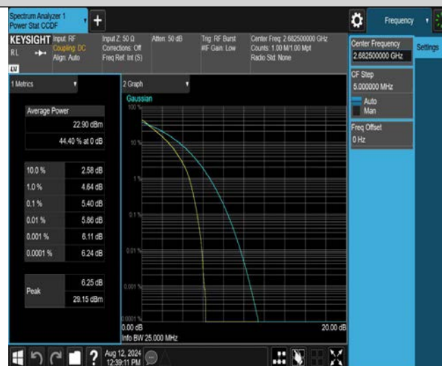
Band41-15MHz-16QAM-39725-1RB#0
