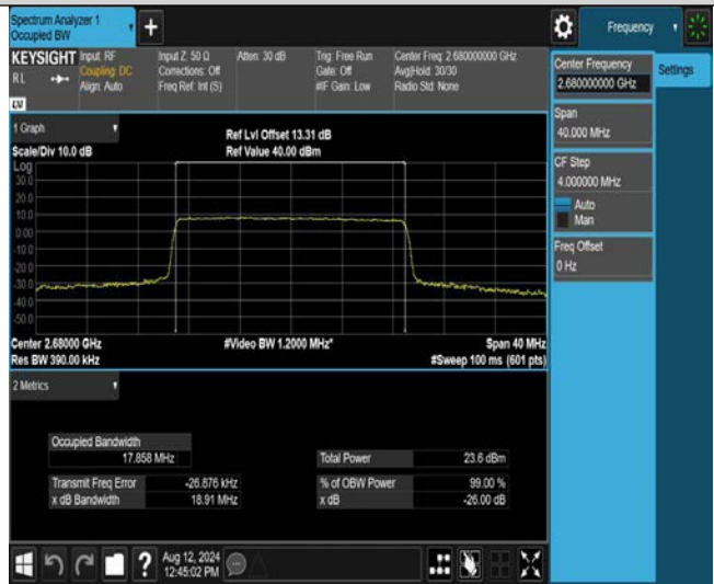
Band41-20MHz-16QAM-39750-100RB#0
