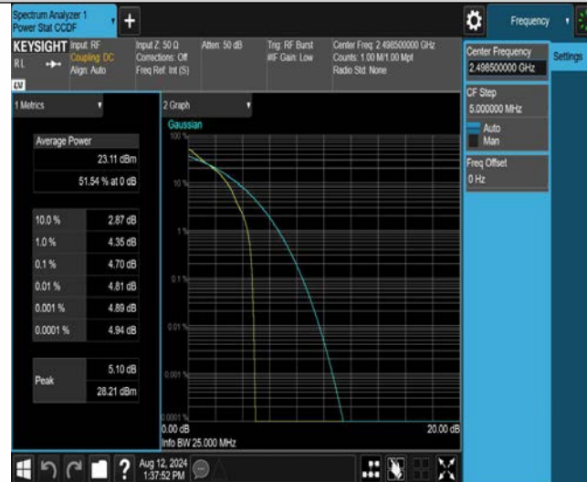
Band41-5MHz-QPSK-39675-25RB#0
