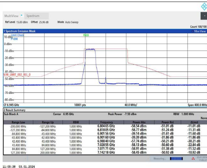
11AX80MIMO Ant2 6945 484Tone RU65
