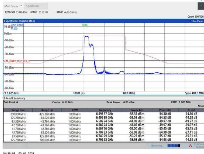
11AX80MIMO Ant1 6625 242Tone RU61
