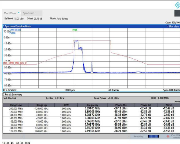
11AX80MIMO Ant2 7025 242Tone RU61
