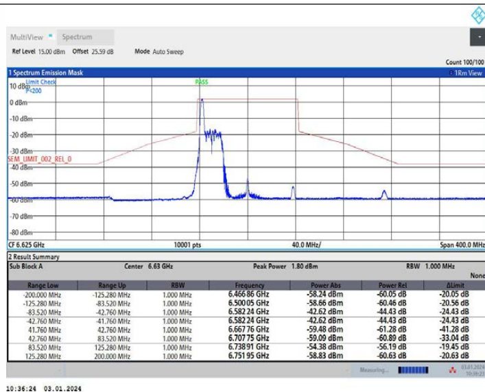
11AX80MIMO Ant1 6625 52Tone RU37
