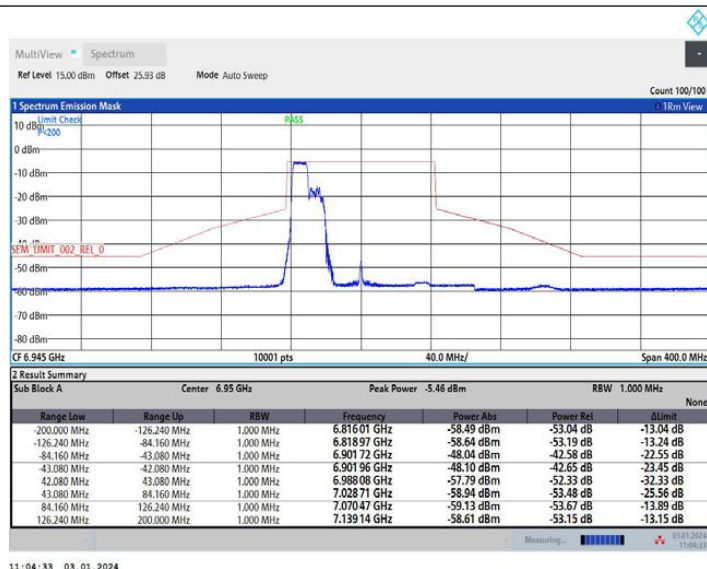
11AX80MIMO Ant1 6945 242Tone RU61
