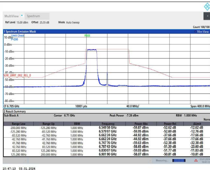
11AX80MIMO Ant2 6705 484Tone RU65
