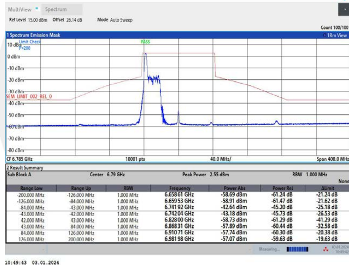
11AX80MIMO Ant2 6785 52Tone RU37
