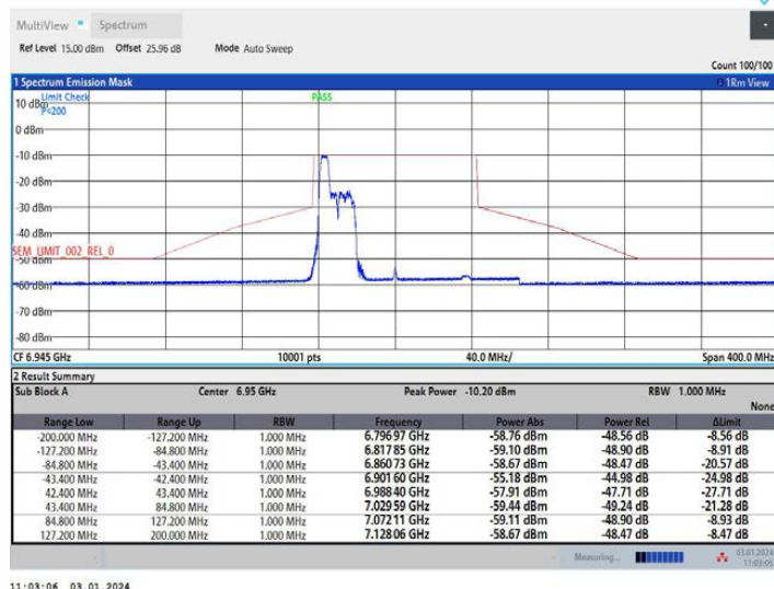
11AX80MIMO Ant2 6945 106Tone RU53
