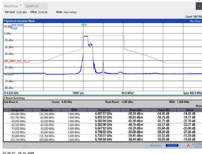
11AX80MIMO Ant2 6625 242Tone RU61
