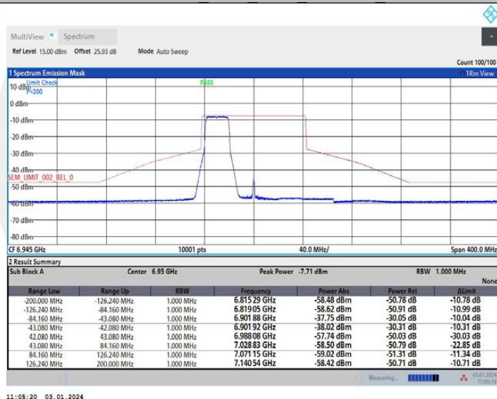
11AX80MIMO Ant1 6945 484Tone RU65
