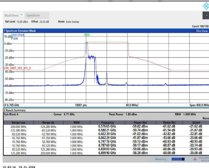
11AX80MIMO Ant2 6705 52Tone RU37
