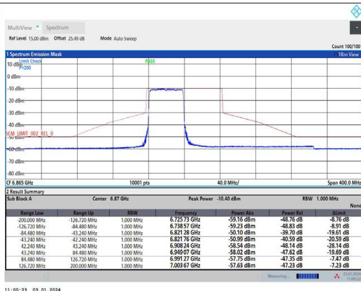
11AX80MIMO Ant2 6865 26Tone RU0
