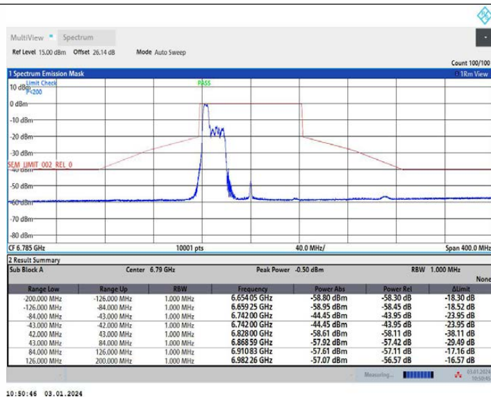
11AX80MIMO Ant2 6785 106Tone RU53
