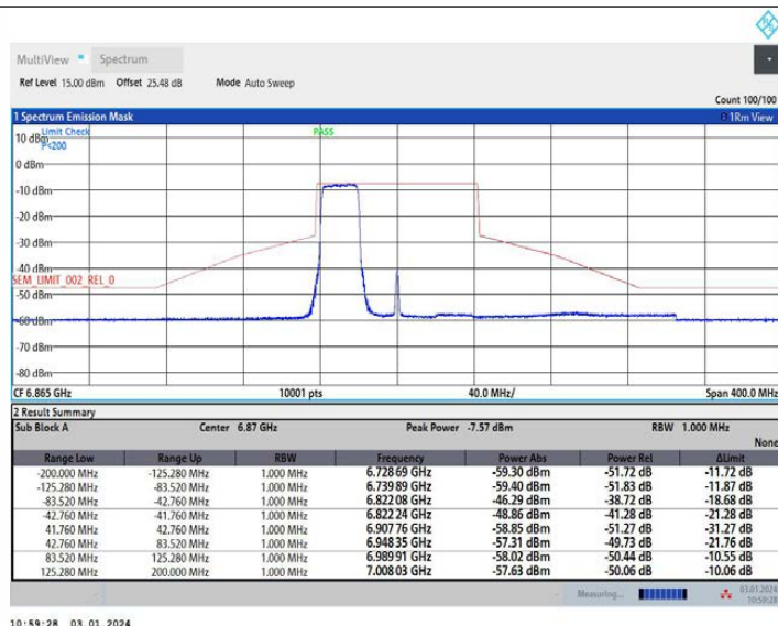
11AX80MIMO Ant2 6865 484Tone RU65
