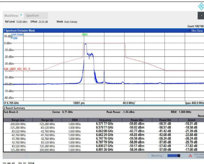
11AX80MIMO Ant2 6705 106Tone RU53
