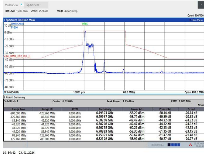
11AX80MIMO Ant2 6625 52Tone RU37
