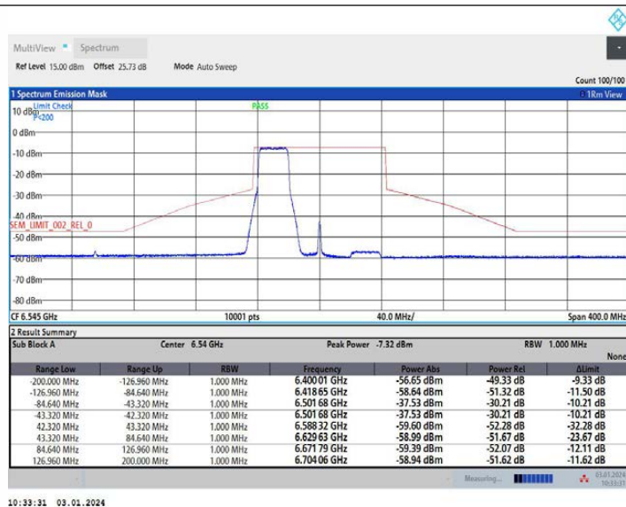
11AX80MIMO Ant2 6545 484Tone RU65
