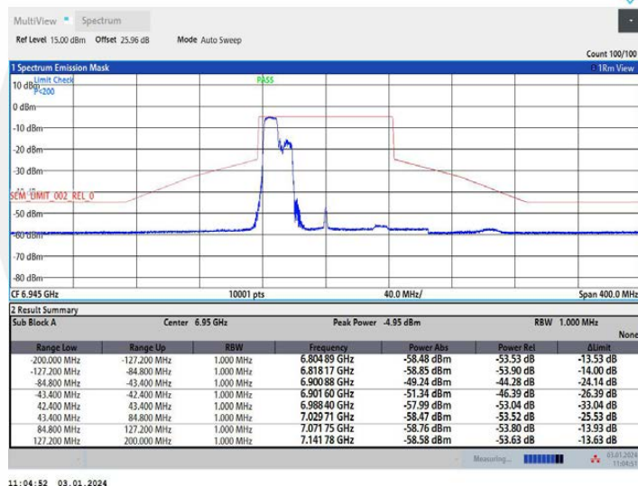
11AX80MIMO Ant2 6945 242Tone RU61
