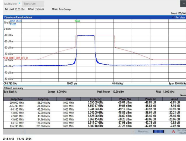
11AX80MIMO Ant2 6785 26Tone RU0
