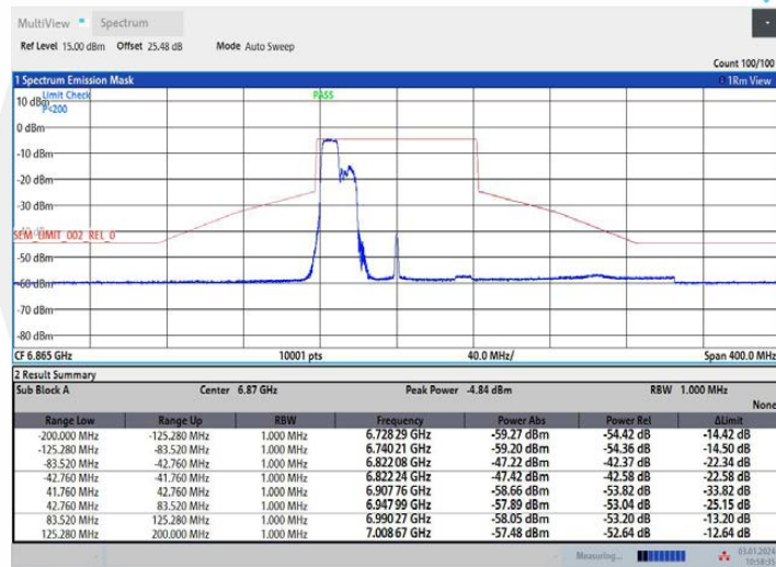
11AX80MIMO Ant2 6865 242Tone RU61
