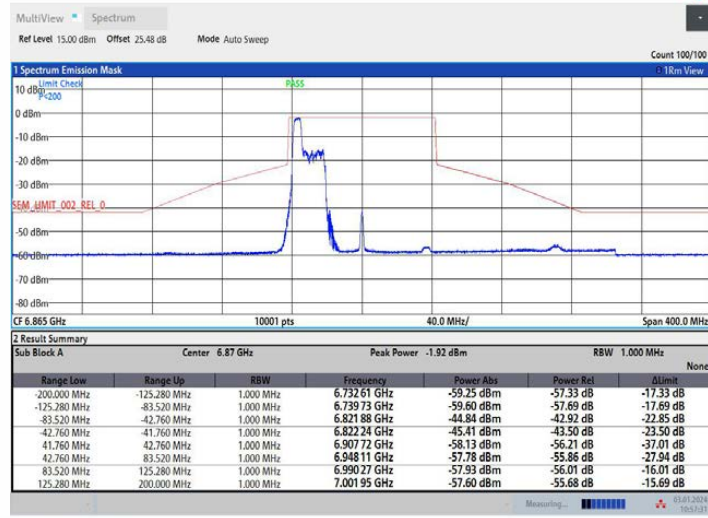
11AX80MIMO Ant2 6865 106Tone RU53
