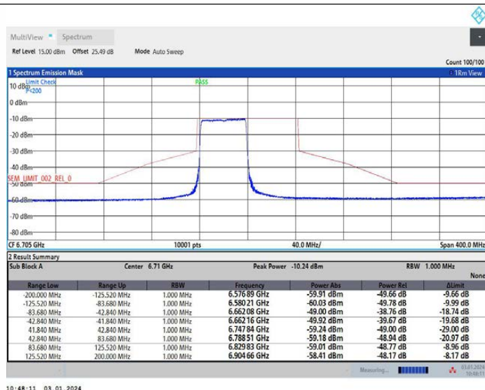
11AX80MIMO Ant2 6705 26Tone RU0
