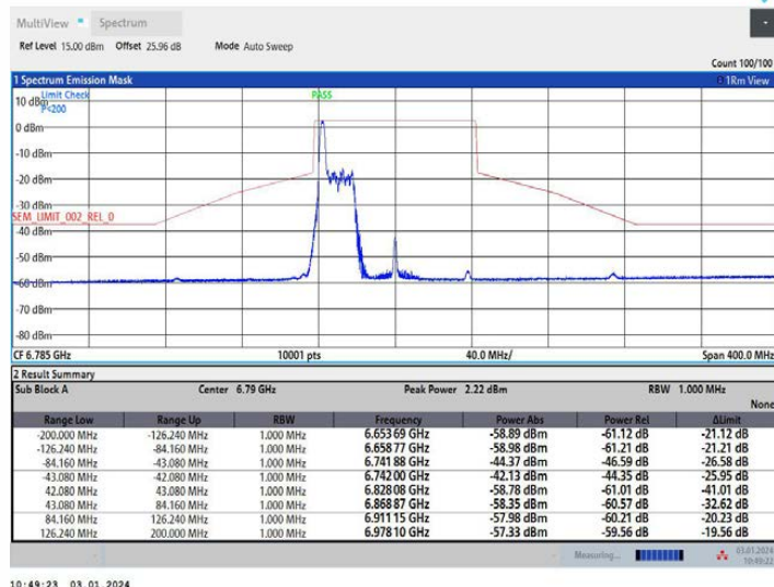
11AX80MIMO Ant1 6785 52Tone RU37
