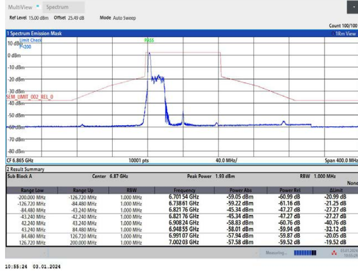
11AX80MIMO Ant1 6865 52Tone RU37
