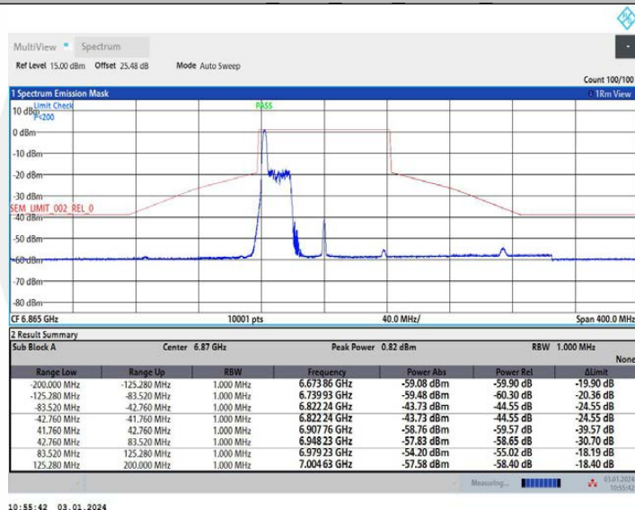
11AX80MIMO Ant2 6865 52Tone RU37
