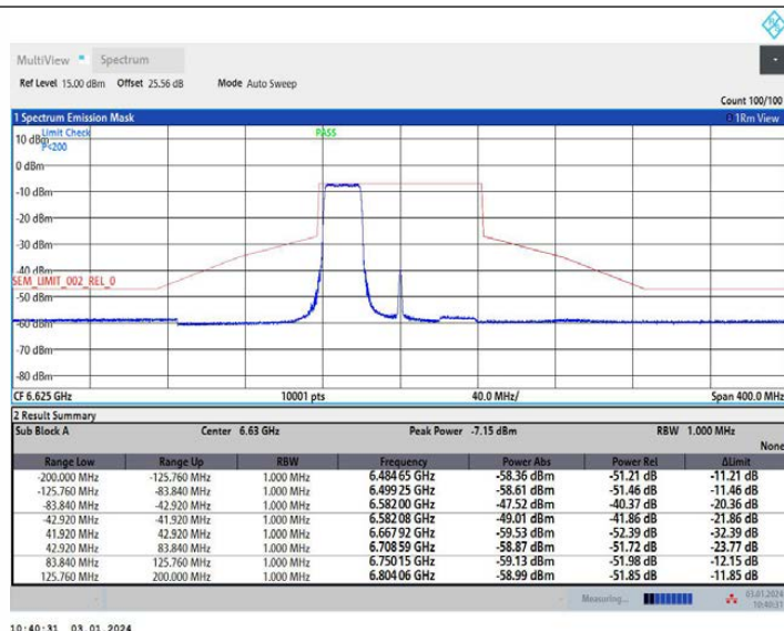
11AX80MIMO Ant2 6625 484Tone RU65
