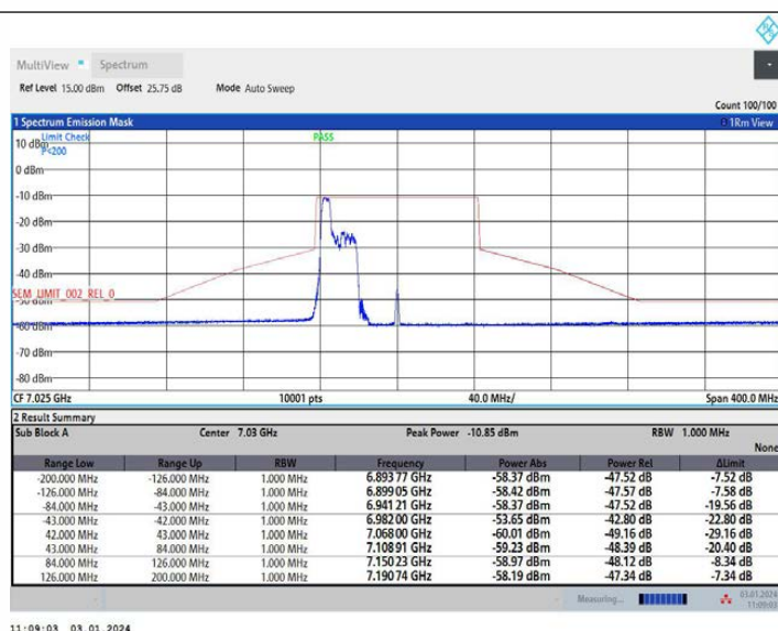
11AX80MIMO Ant2 7025 106Tone RU53
