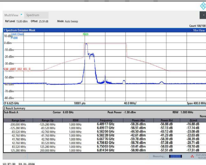
11AX80MIMO Ant1 6625 106Tone RU53
