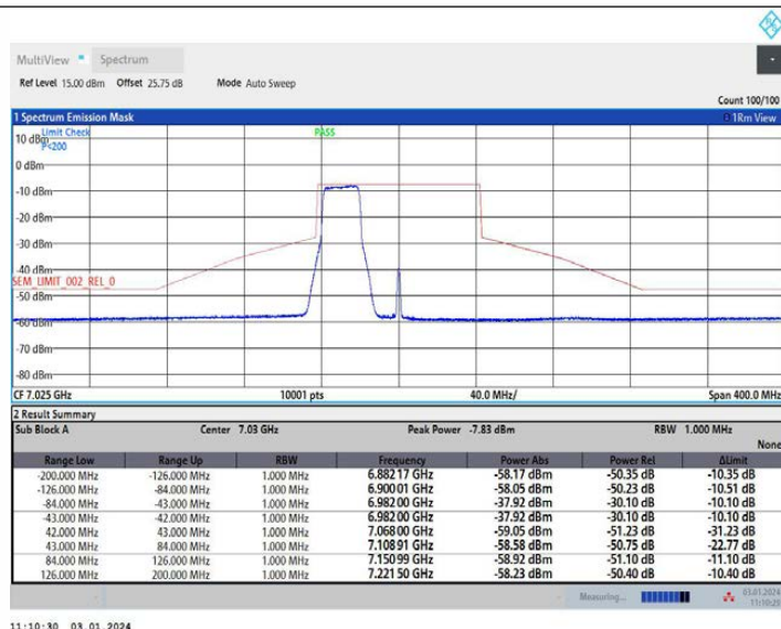
11AX80MIMO Ant2 7025 484Tone RU65
