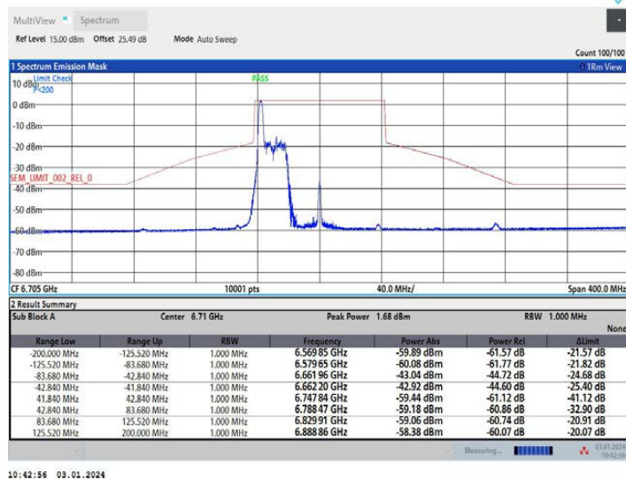
11AX80MIMO Ant1 6705 52Tone RU37
