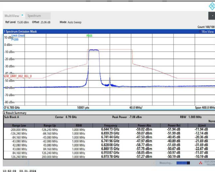
11AX80MIMO Ant1 6785 484Tone RU65
