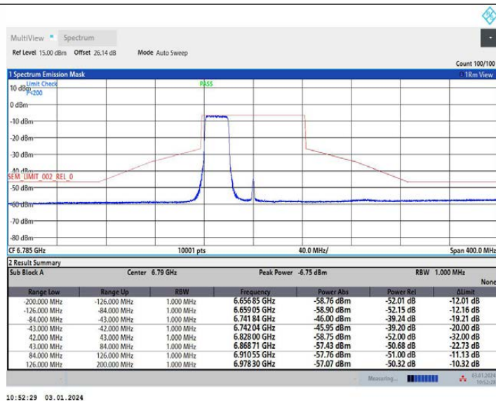
11AX80MIMO Ant2 6785 484Tone RU65
