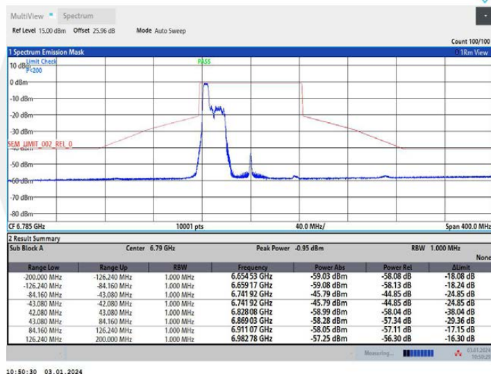
11AX80MIMO Ant1 6785 106Tone RU53
