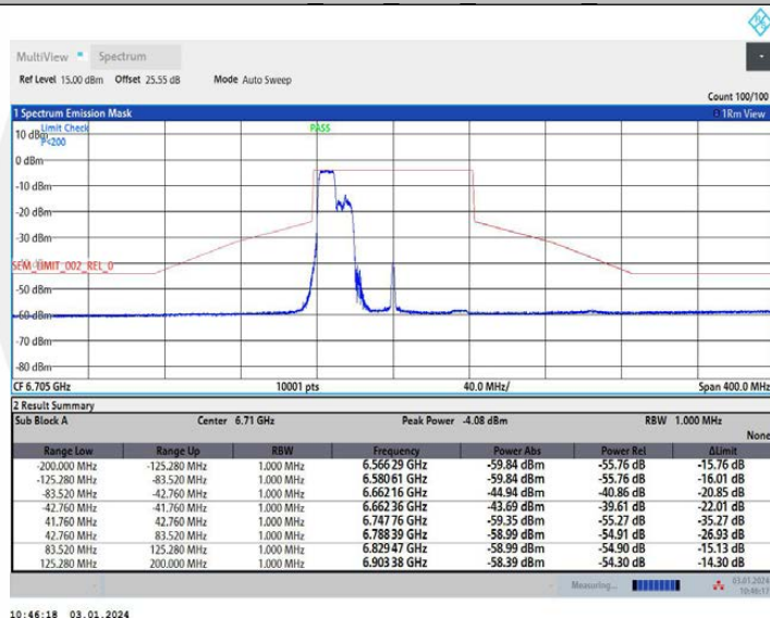
11AX80MIMO Ant2 6705 242Tone RU61
