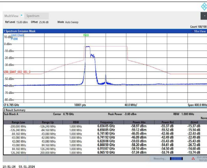
11AX80MIMO Ant1 6785 242Tone RU61
