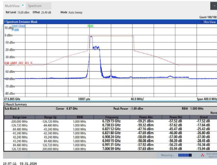
11AX80MIMO Ant1 6865 106Tone RU53
