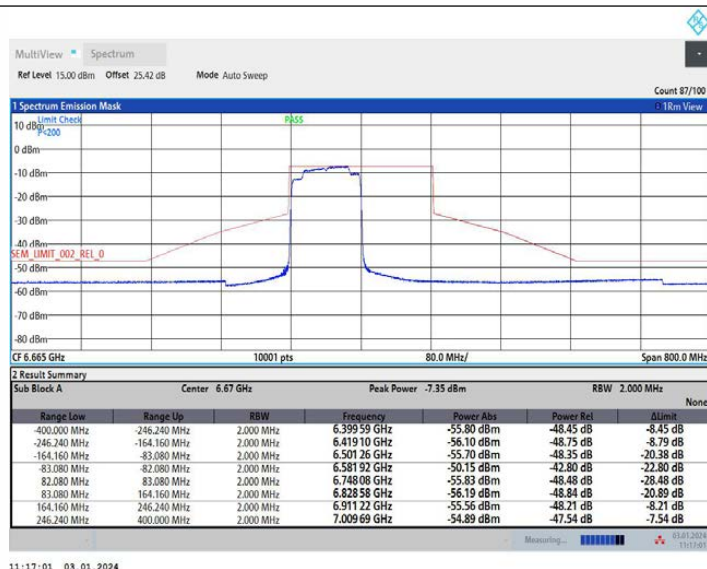
11AX160MIMO Ant2 6665 996Tone RU67
