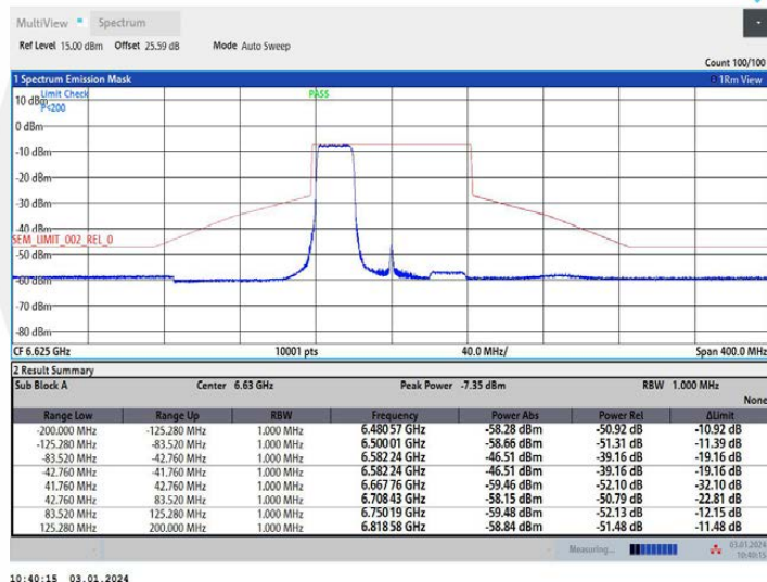
11AX80MIMO Ant1 6625 484Tone RU65
