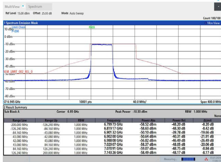
11AX80MIMO Ant2 6945 26Tone RU0
