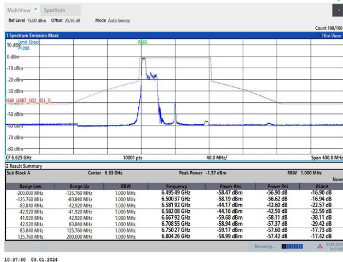
11AX80MIMO Ant2 6625 106Tone RU53
