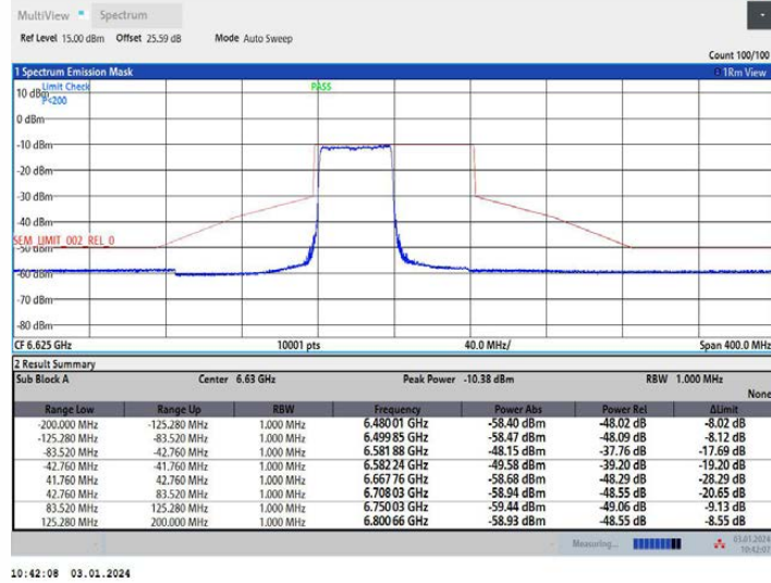
11AX80MIMO Ant2 6625 26Tone RU0
