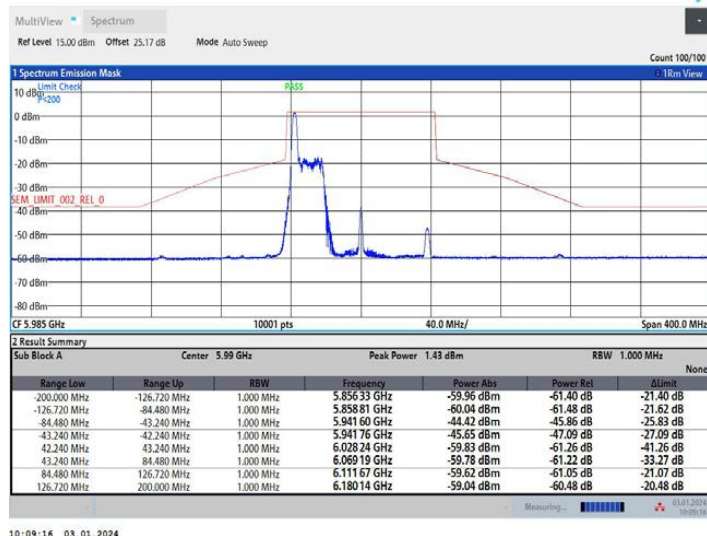
11AX80MIMO Ant1 5985 52Tone RU37
