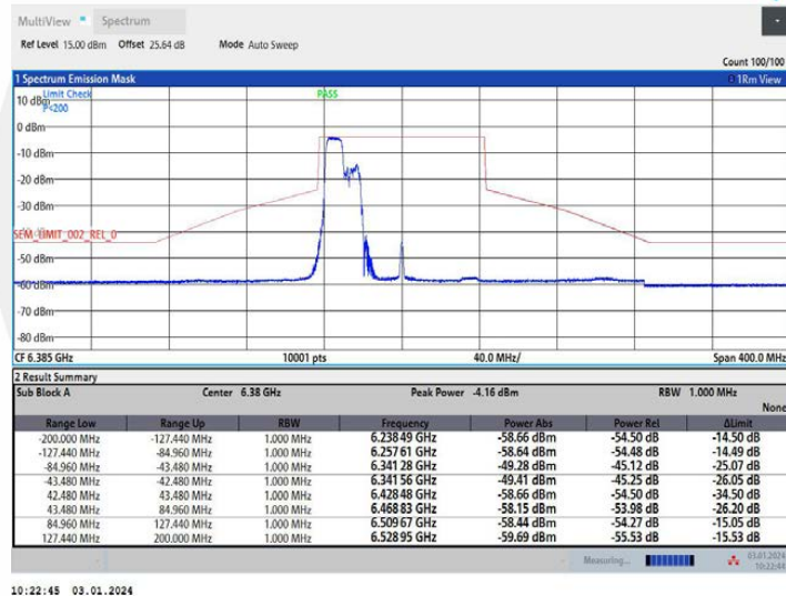
11AX80MIMO Ant2 6385 242Tone RU61
