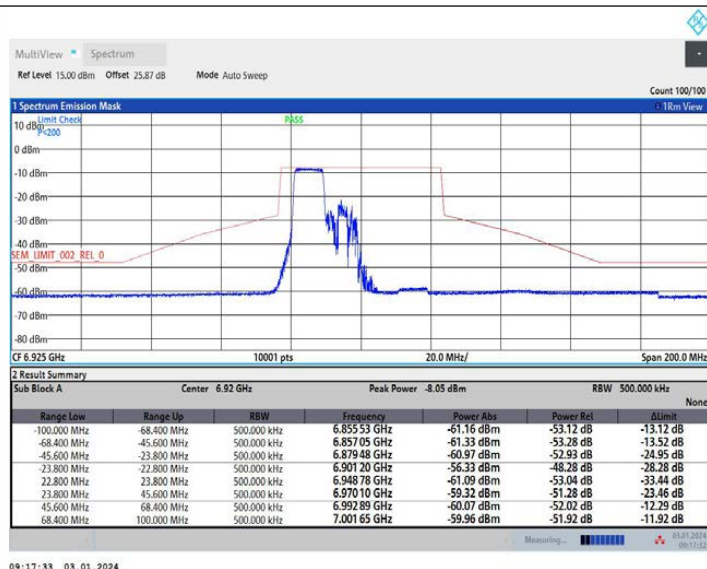
11AX40MIMO Ant2 6925 242Tone RU61
