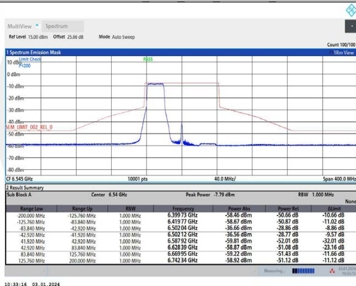
11AX80MIMO Ant1 6545 484Tone RU65
