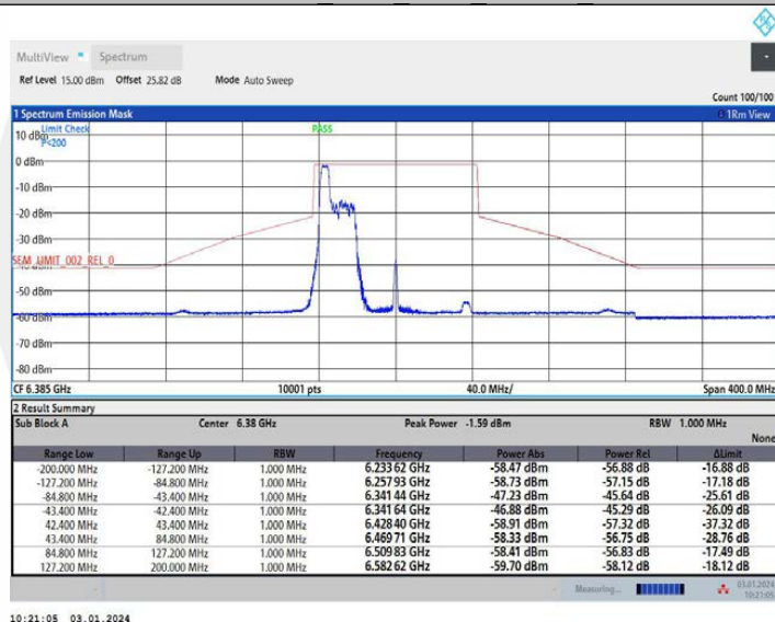
11AX80MIMO Ant1 6385 106Tone RU53
