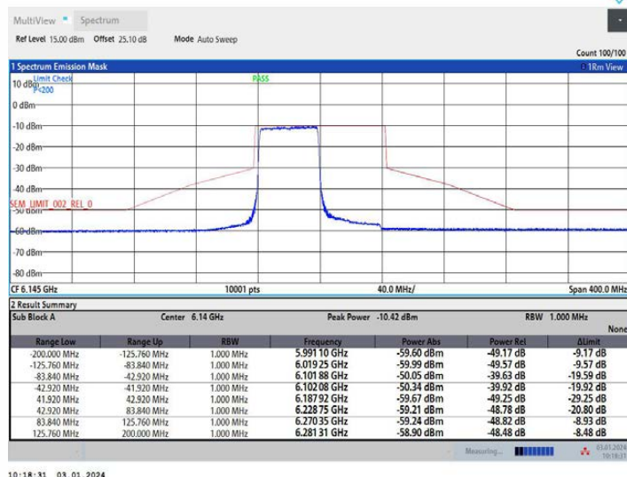
11AX80MIMO Ant2 6145 26Tone RU0
