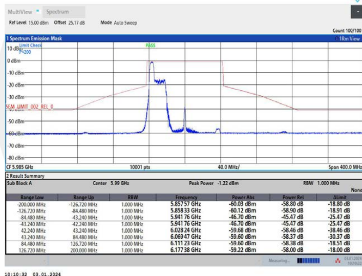
11AX80MIMO Ant1 5985 106Tone RU53
