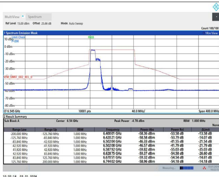
11AX80MIMO Ant1 6545 242Tone RU61
