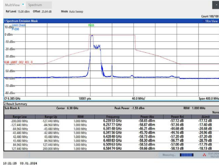
11AX80MIMO Ant2 6385 106Tone RU53
