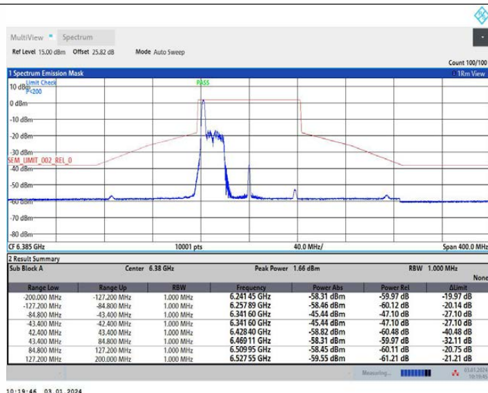
11AX80MIMO Ant1 6385 52Tone RU37
