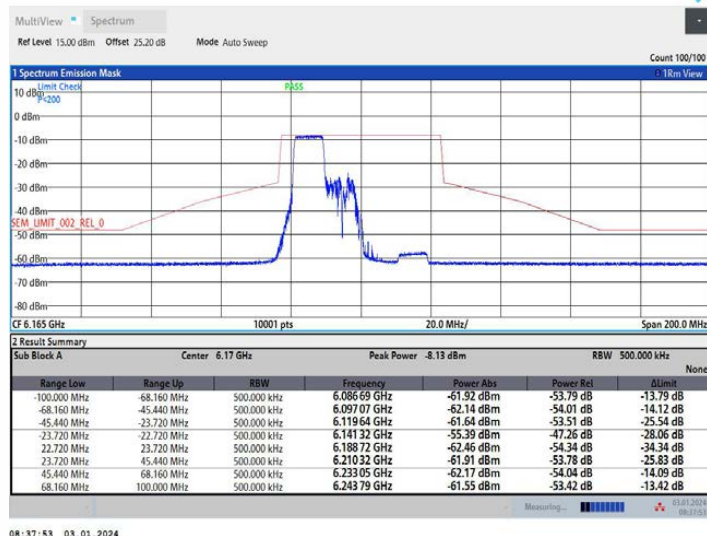
11AX40MIMO Ant2 6165 242Tone RU61
