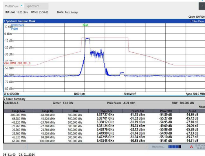
11AX40MIMO Ant2 6405 106Tone RU53
