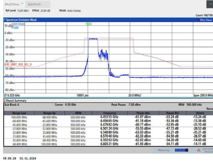
11AX40MIMO Ant2 6525 242Tone RU61
