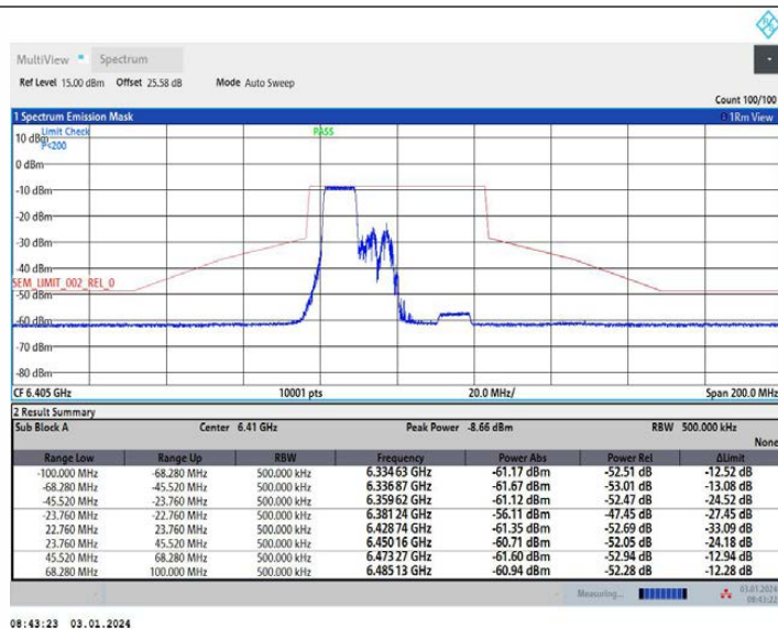
11AX40MIMO Ant2 6405 242Tone RU61
