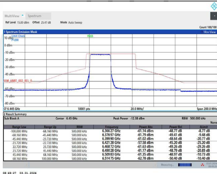
11AX40MIMO Ant2 6445 26Tone RU0
