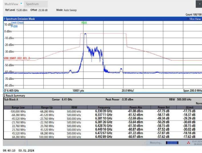
11AX40MIMO Ant2 6405 52Tone RU37
