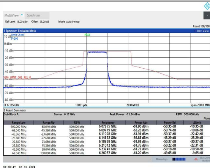
11AX40MIMO Ant2 6165 26Tone RU0
