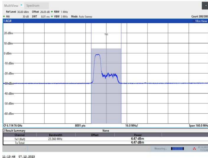
11AX80MIMO_Ant1_6145_106Tone_RU53
