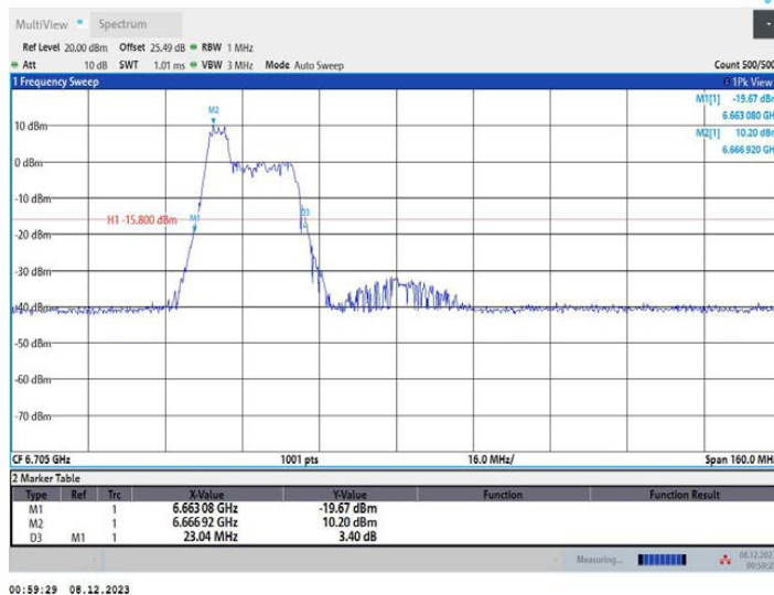
11AX80MIMO_Ant1_6705_106Tone_RU53
