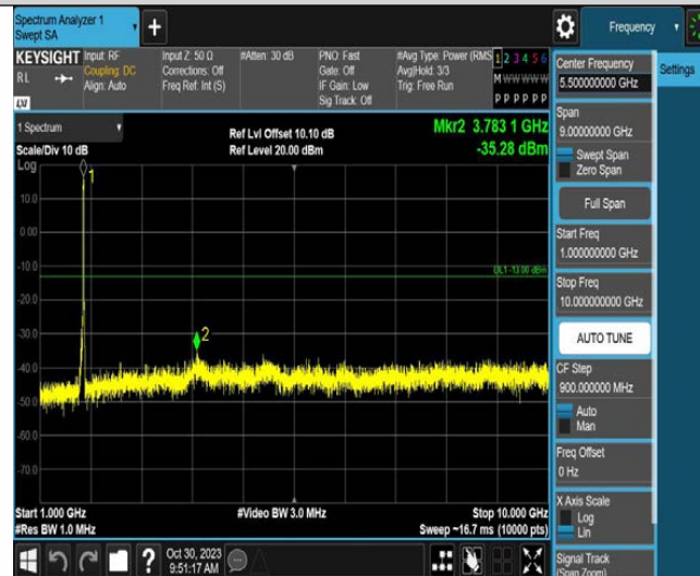
Band66-20MHz-64QAM-132572-100RB#0-Range2:1000~10000MHz
