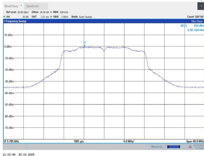
11A_Ant1_5785
