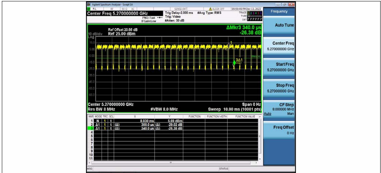
11AX40MIMO Ant2 5270
