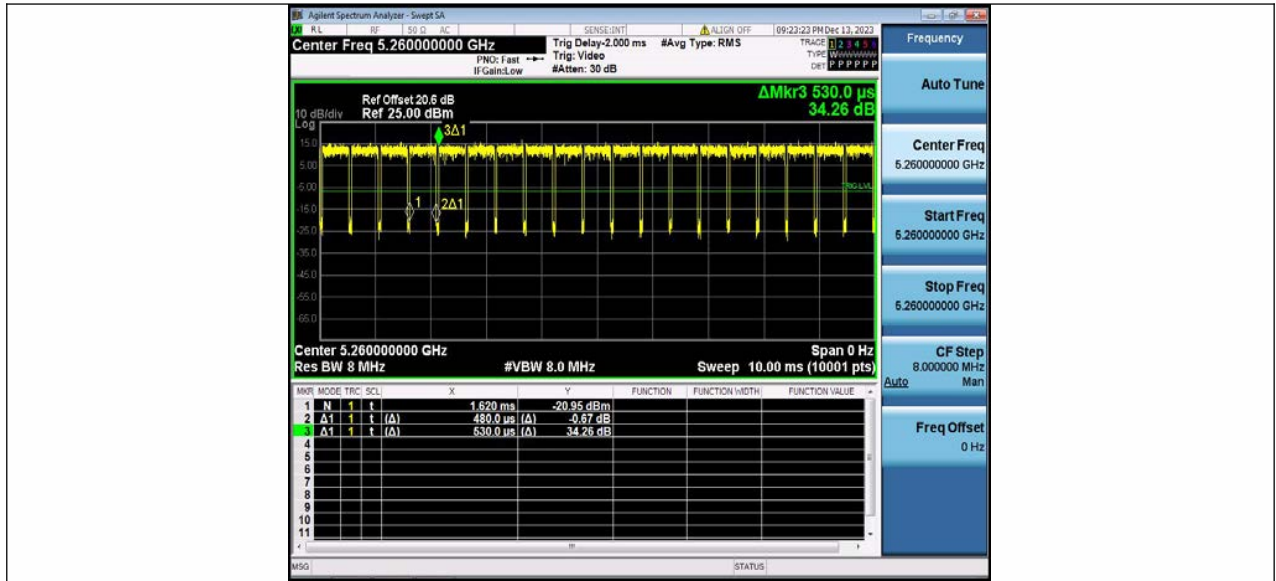
11AX20MIMO Ant2 5260
