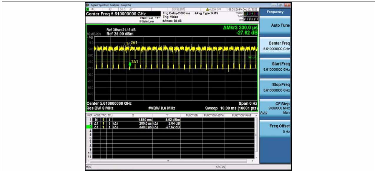
11AC80MIMO Ant2 5610
