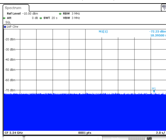
Without Data Traffic Plot (Noise Plot)
