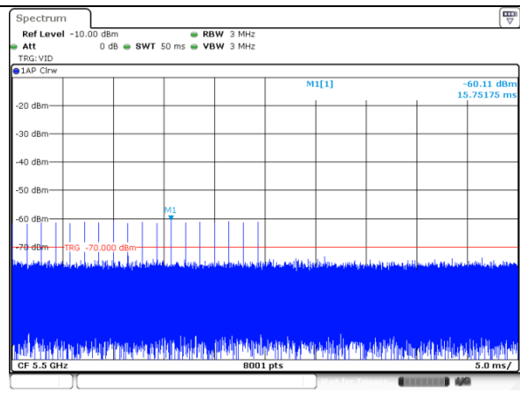
Calibration Radar # 0 detection threshold level
