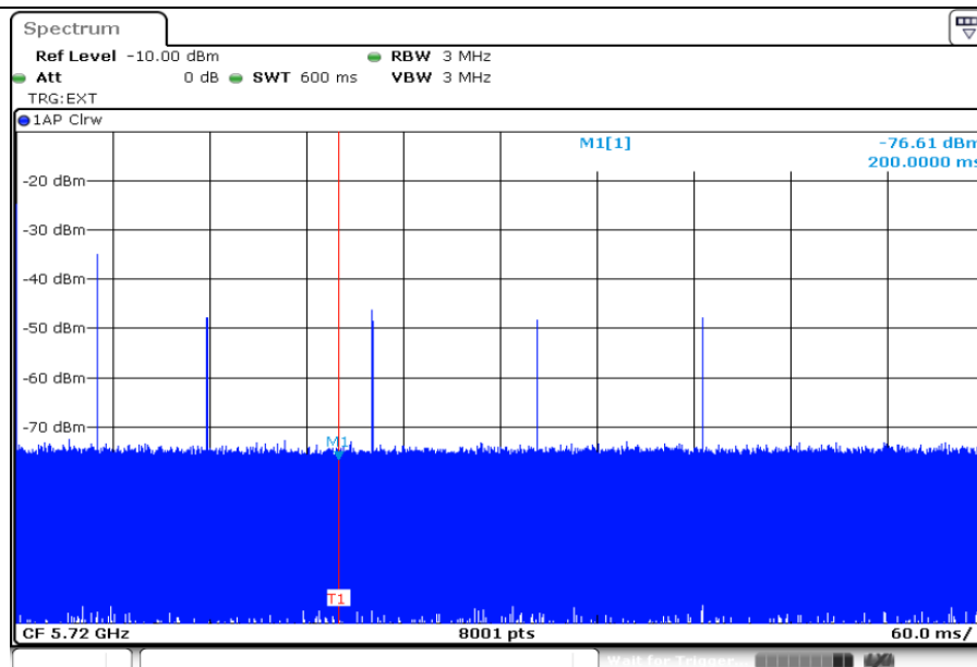
Zoom-in 600 ms Timing Plot
