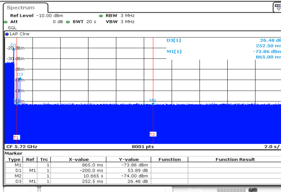
20 sec Timing Plot
