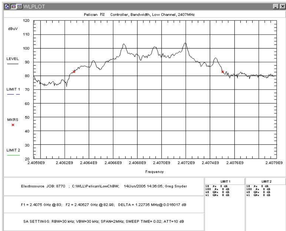
Figure 1. Occupied Bandwidth, Low Channel
