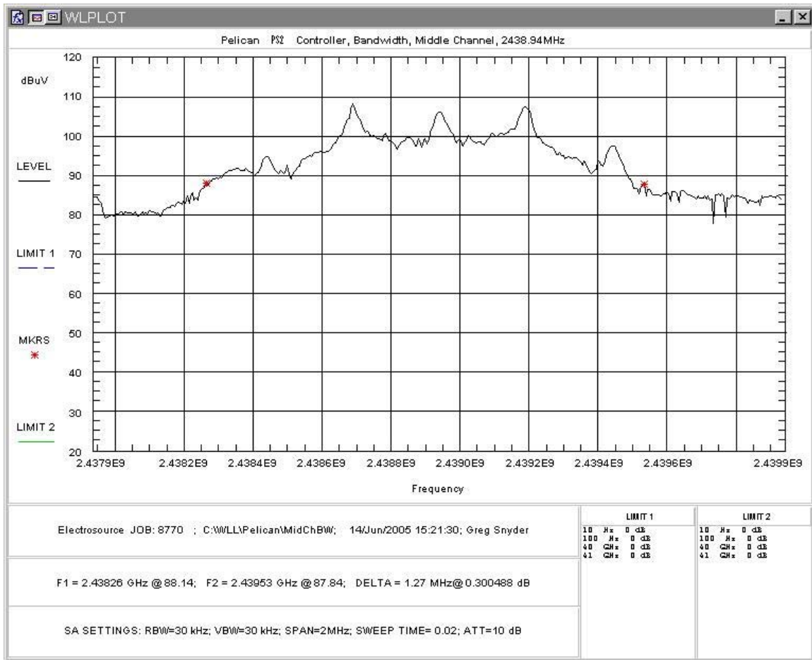
Figure 2. Occupied Bandwidth, Mid Channel
