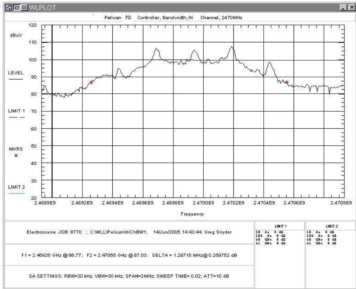
Figure 3. Occupied Bandwidth, High Channel
