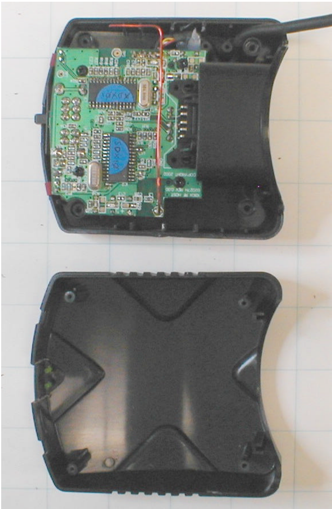
Cover Removed
