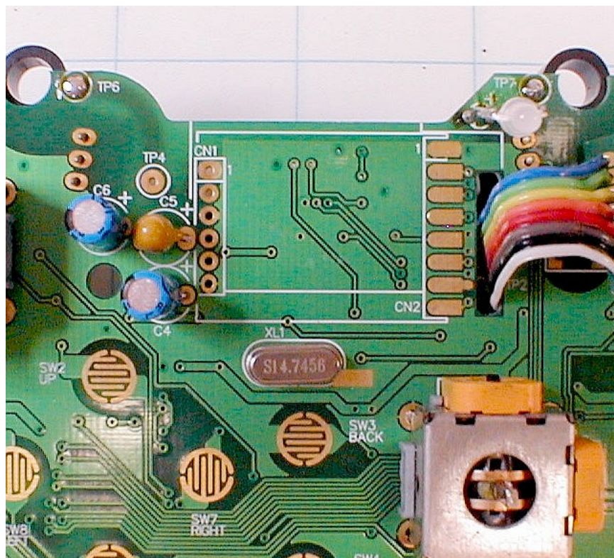
ANT Module Removed
