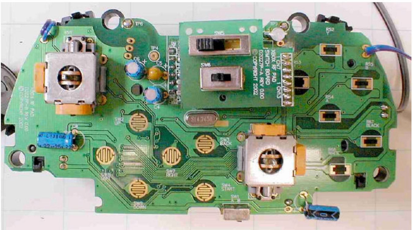
Board Bottom (Switch PCB in place)
