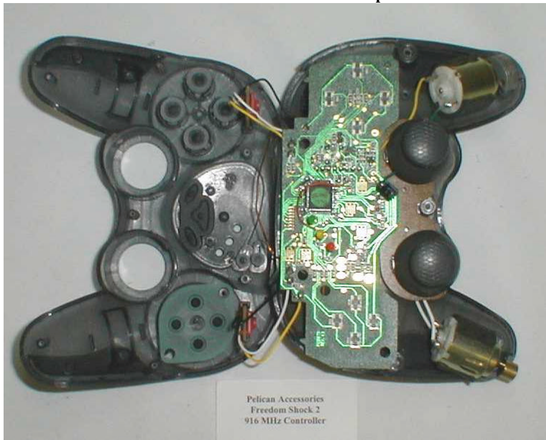
Internal View Top
