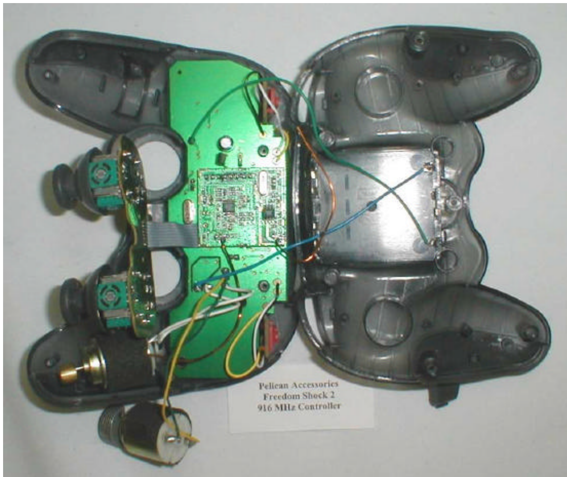
Internal View Bottom
