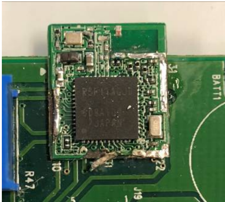
Figure 1. Component Side of BLE Module, Shielding Removed
