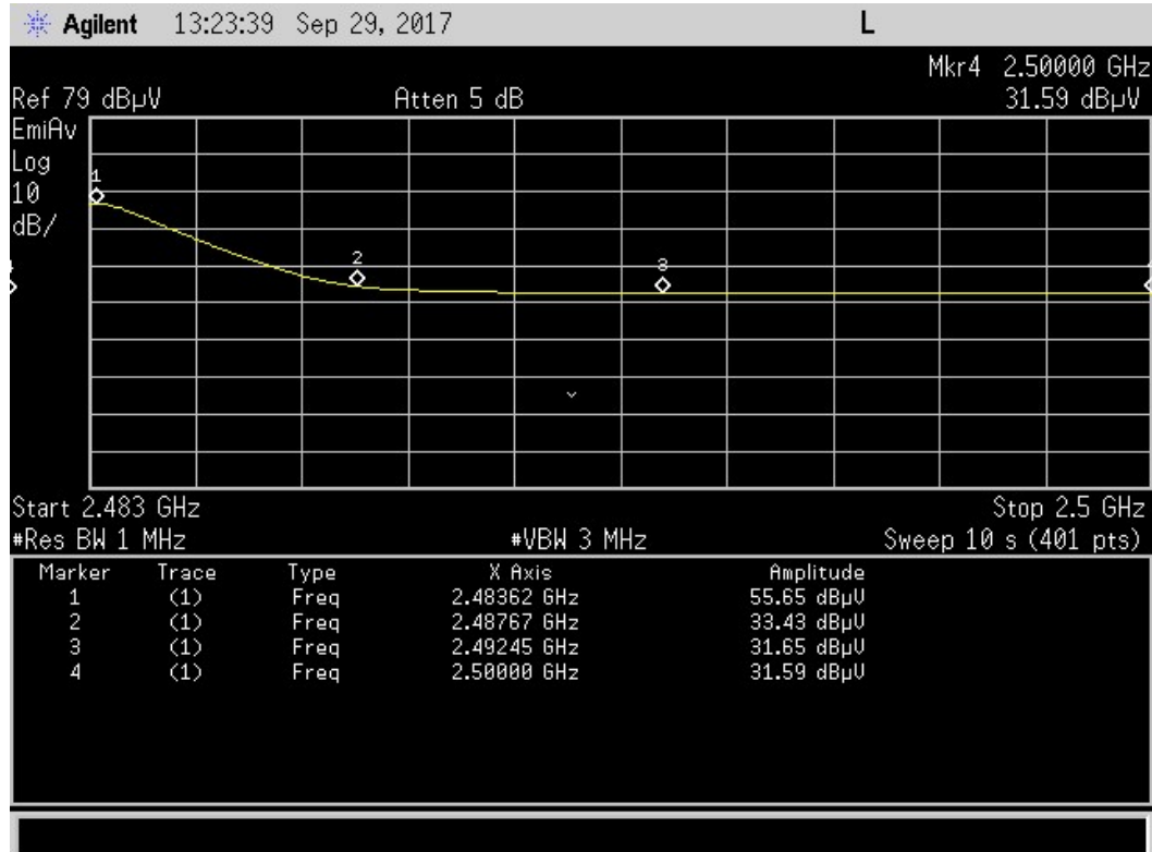
Figure 17. Radiated Restricted Band 2483.5 MHz to 2500 MHz, Average
