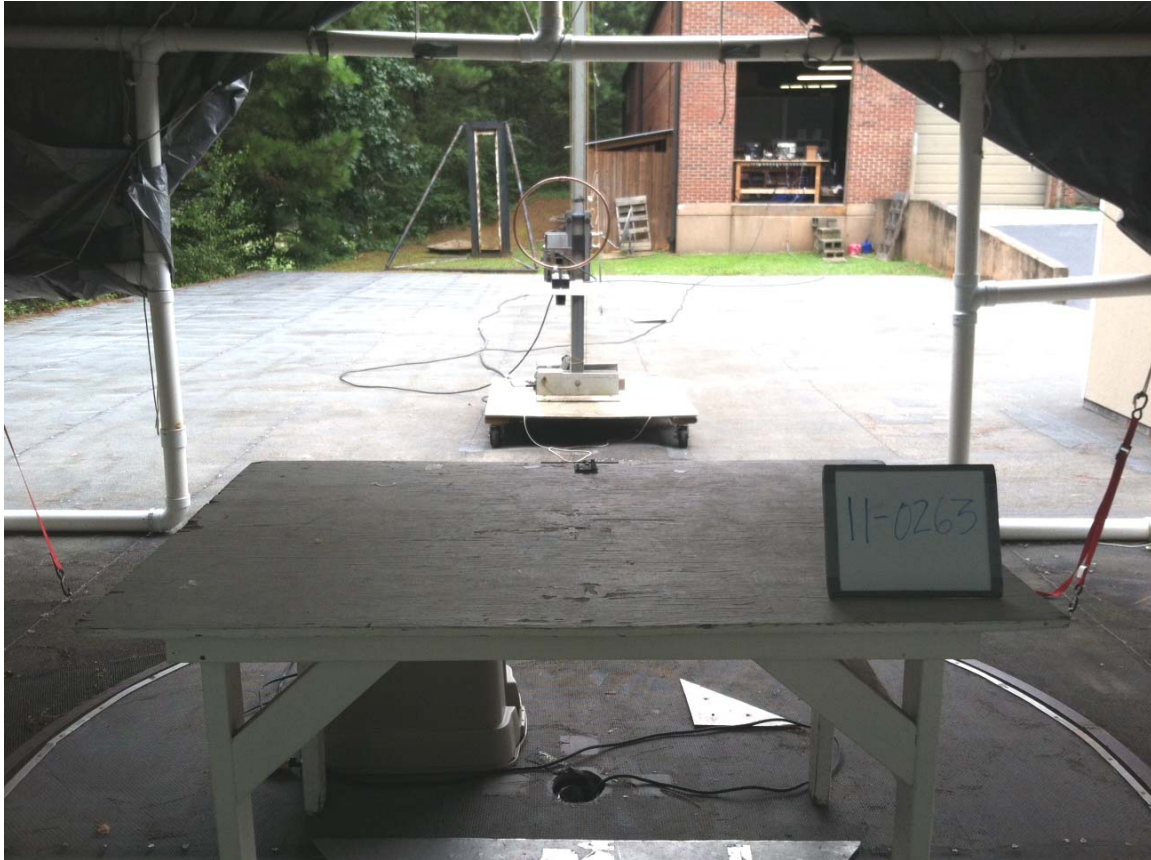
Figure 4- Test Setup, Loop Antenna
