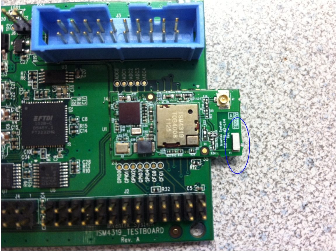
Figure 2- Radio Module with u.fl and Chip Antenna - Top View
