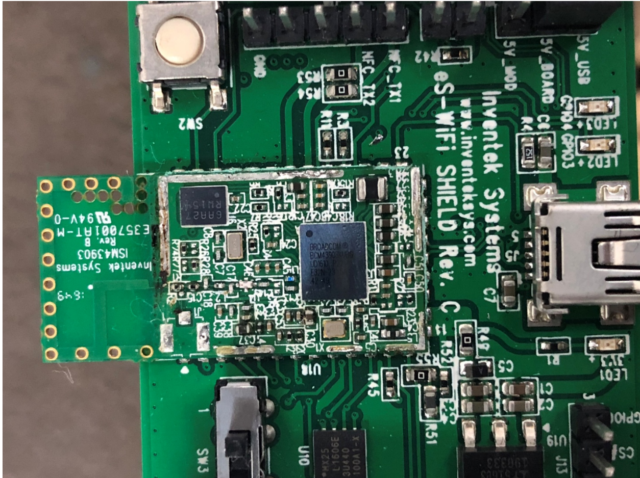
Figure 1. 2.4 GHz ISM Radio on Evaluation Board
