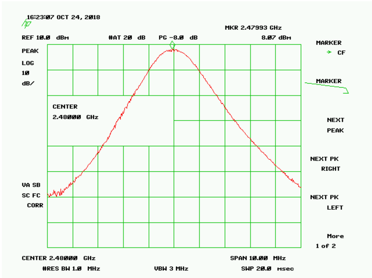
Figure 20. Peak Antenna Conducted Output Power, High Channel
