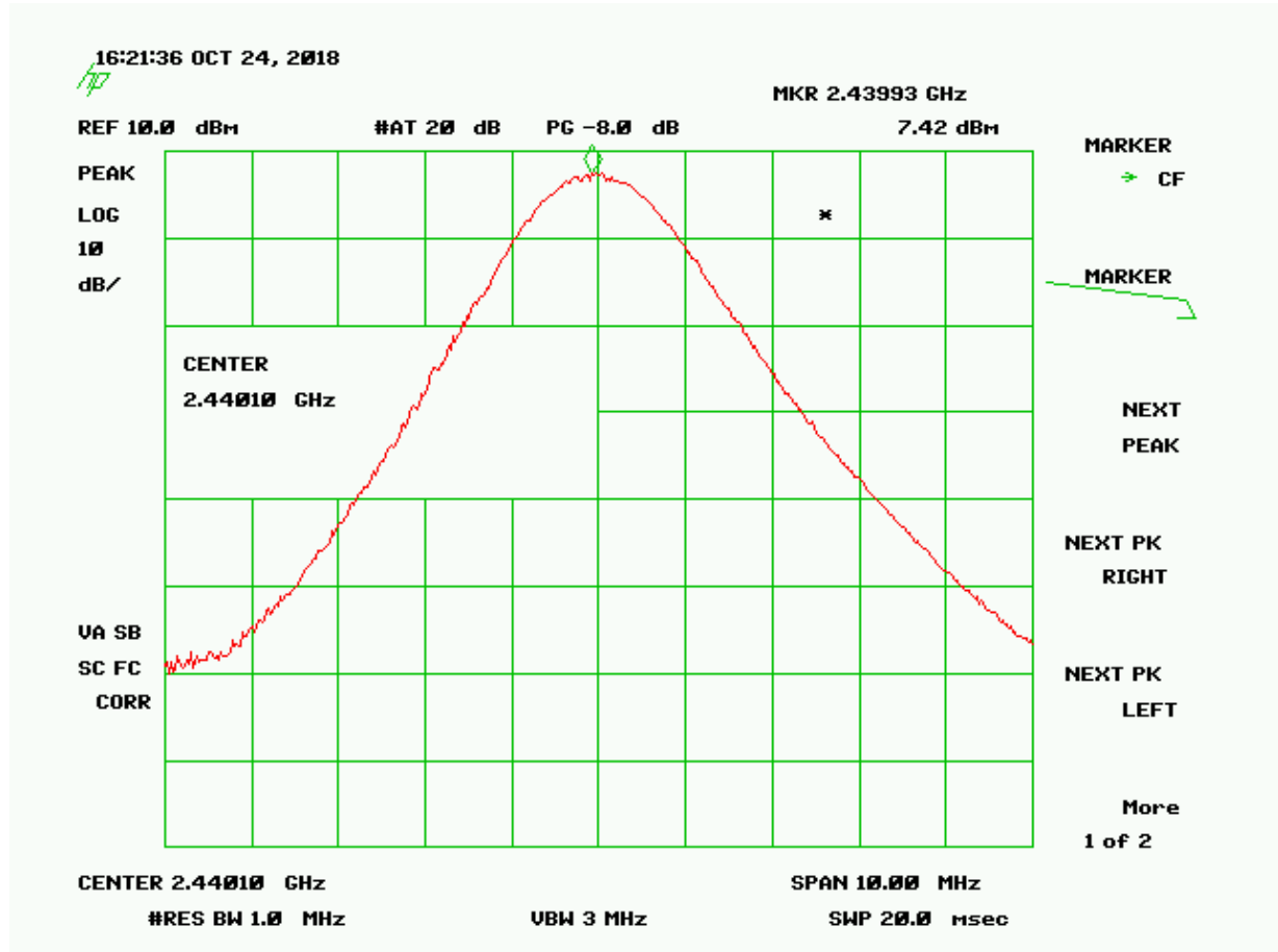
Figure 19. Peak Antenna Conducted Output Power, Mid Channel
