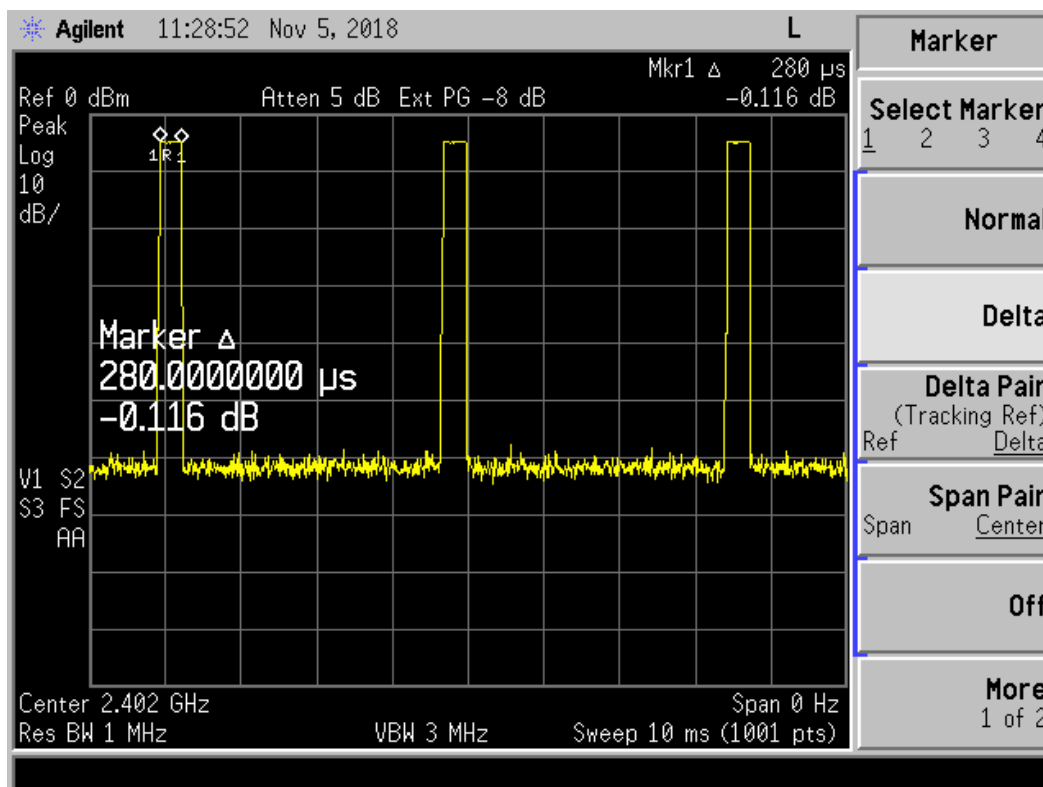
Figure 23. Time of Occupancy
