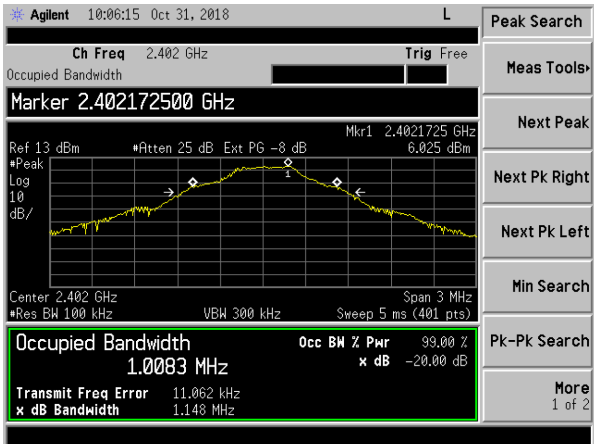
Figure 15. 99% & Twenty dB Bandwidth – Low Channel
