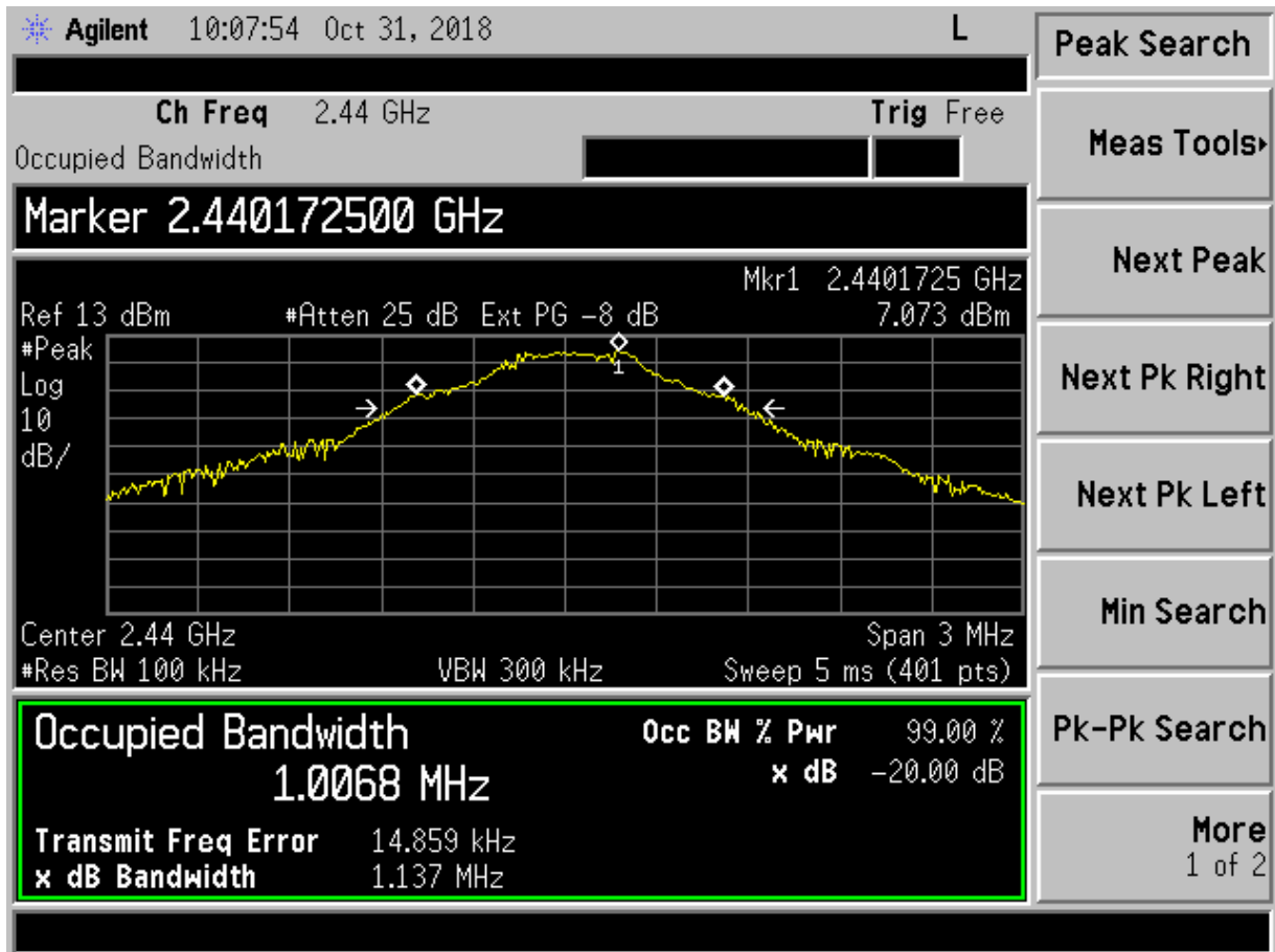
Figure 16. 99% & Twenty dB Bandwidth – Mid Channel
