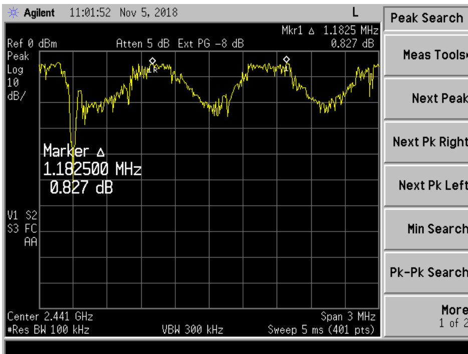
Figure 22. Channel Separation
