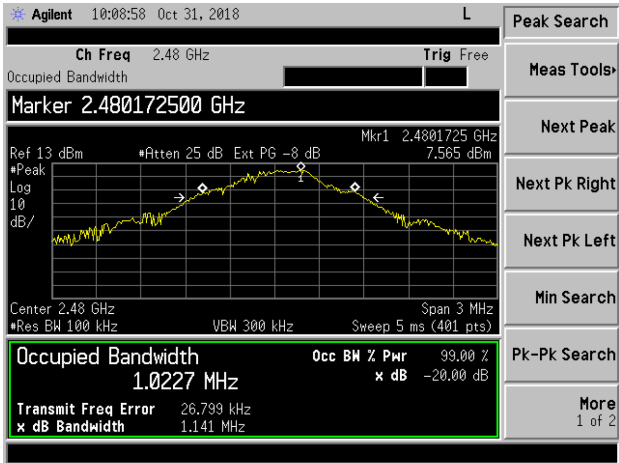
Figure 17. 99% & Twenty dB Bandwidth – High Channel
