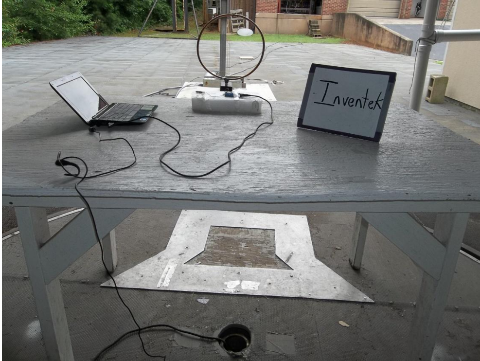
Figure 4- Radiated Emissions, Loop Antenna
