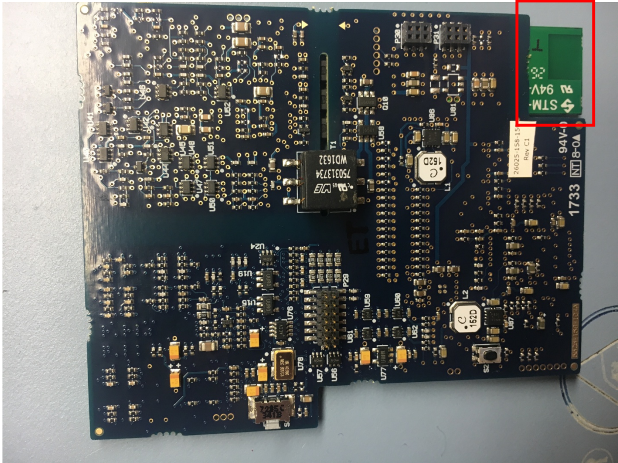
Bottom of Host Device PCB, with bottom of Module Board Outlined
