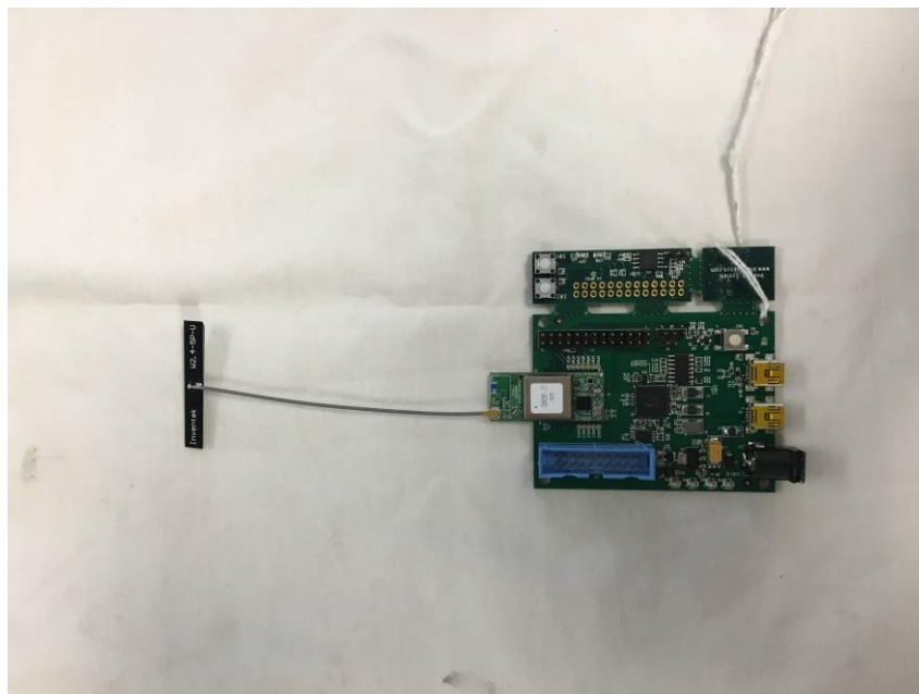
Figure 2. Radiated Emissions (Module with WiFi+BT only)
