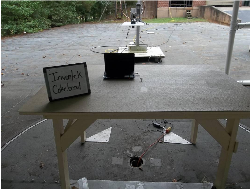
Figure 3. Radiated Emissions Test Setup using Module with WiFi+BT+NFC 0.15 MHz to 30 MHz
