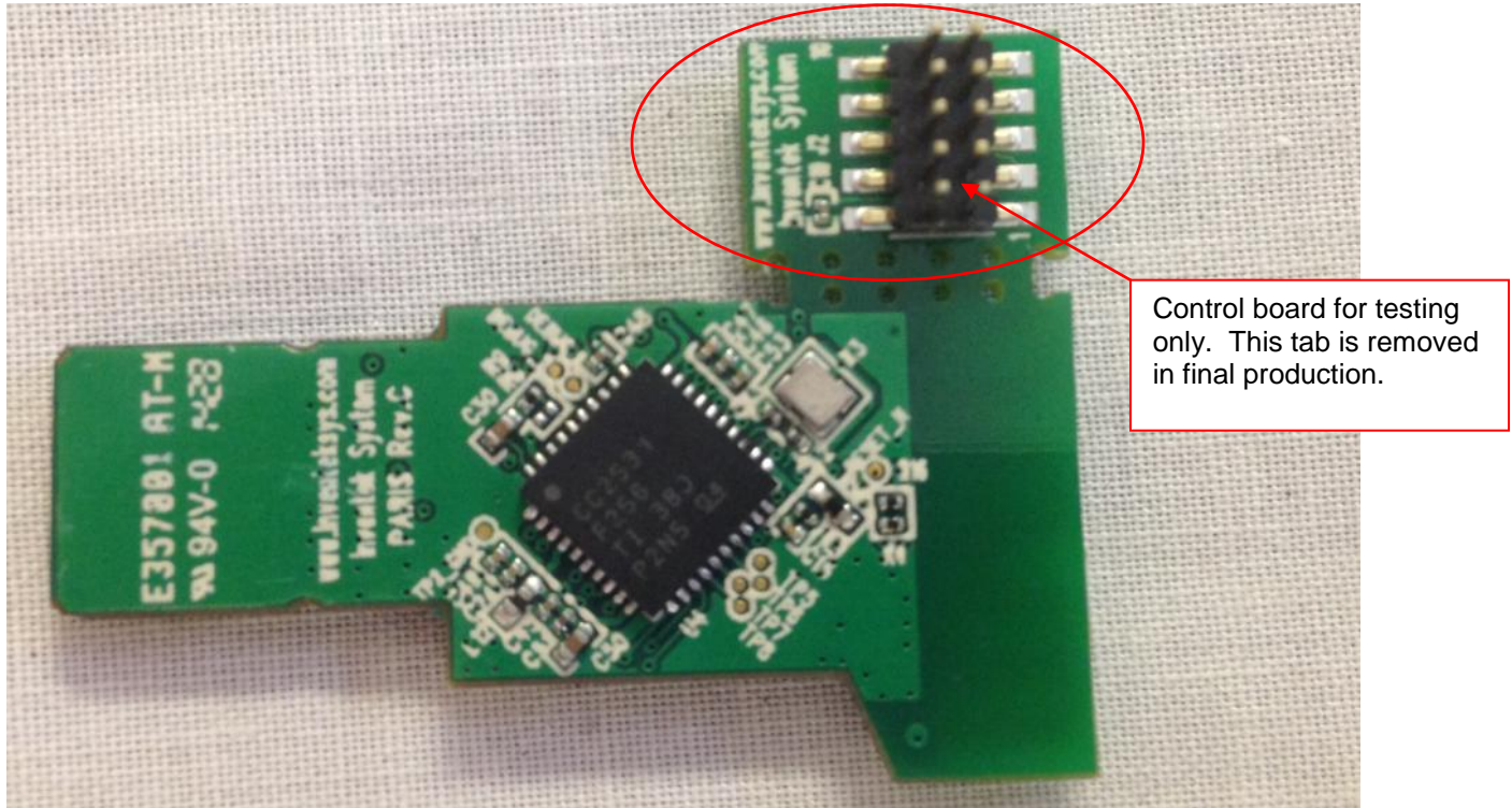
Photo 1 – Top of EUT
