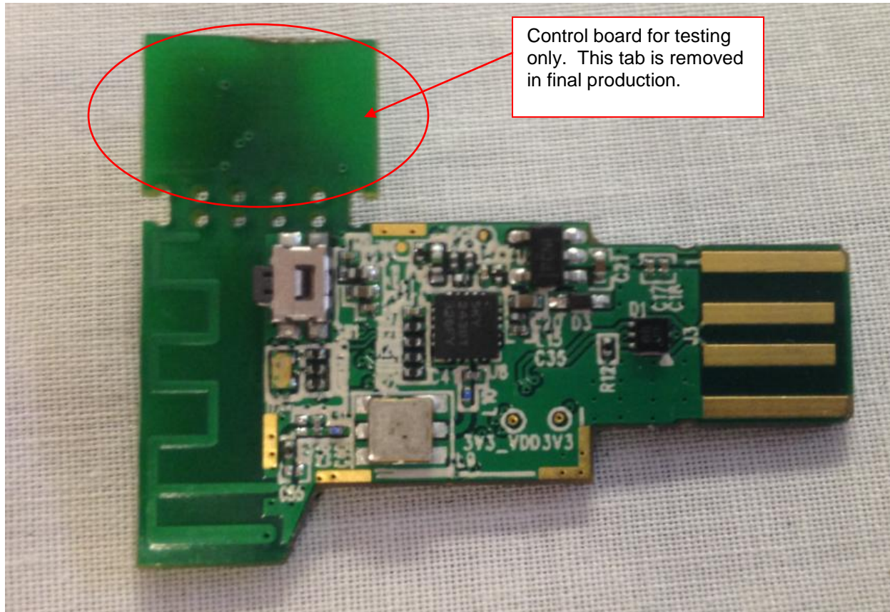
Photo 2 – Back of EUT
