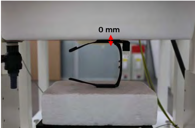
Fig.3 Position the outside of the arm against the phantom(Plot 1)
