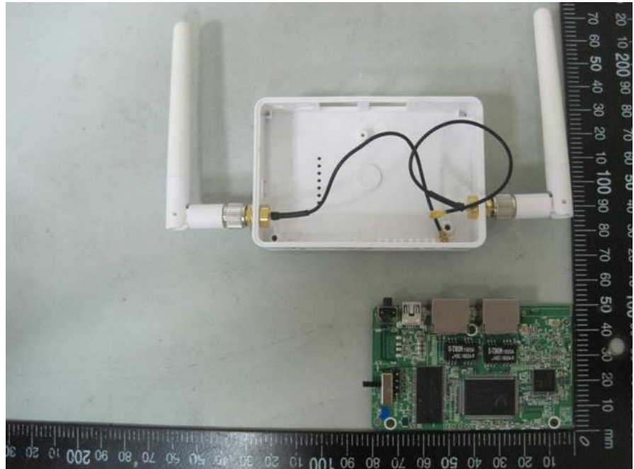
EUT 1. EUT with Dipole Antenna
