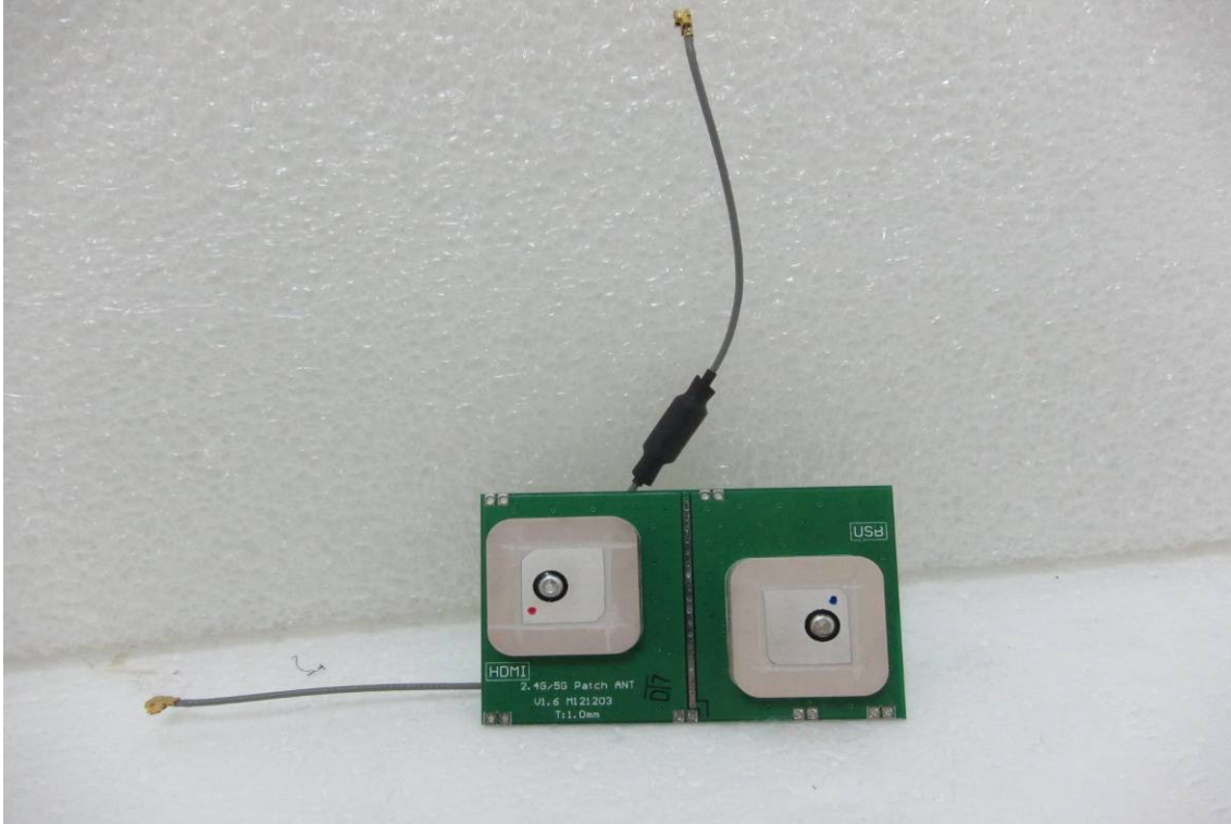
EUT 11 (antenna 3-3)
