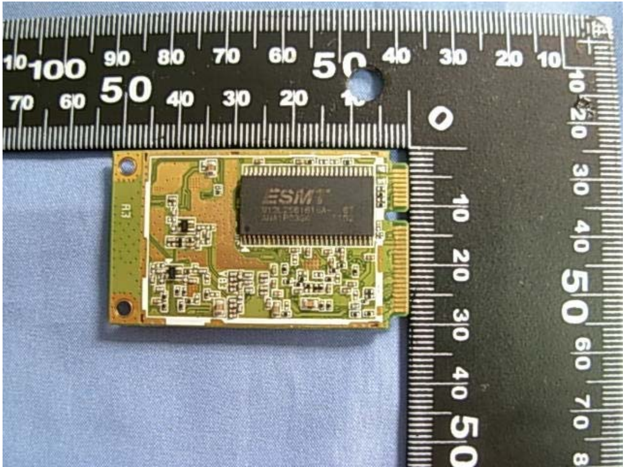
(3) EUT Photo (MB)
