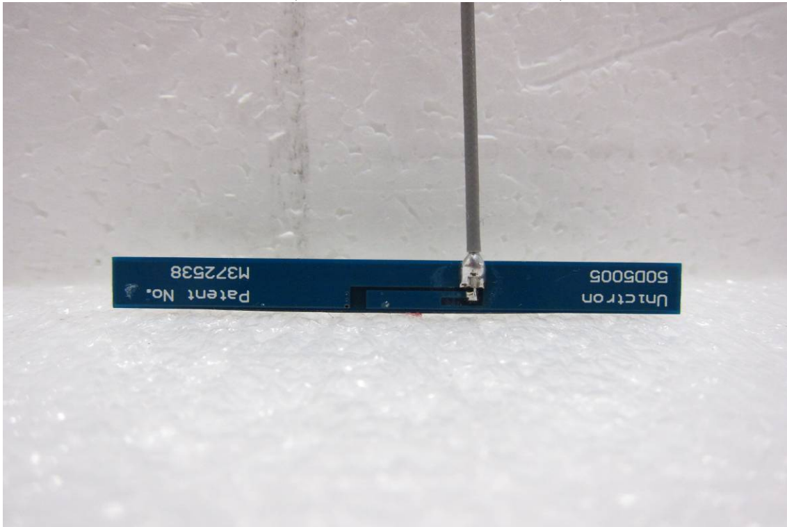
ANT 6 (H2P566WKBA0100 / 2.3dBi)
