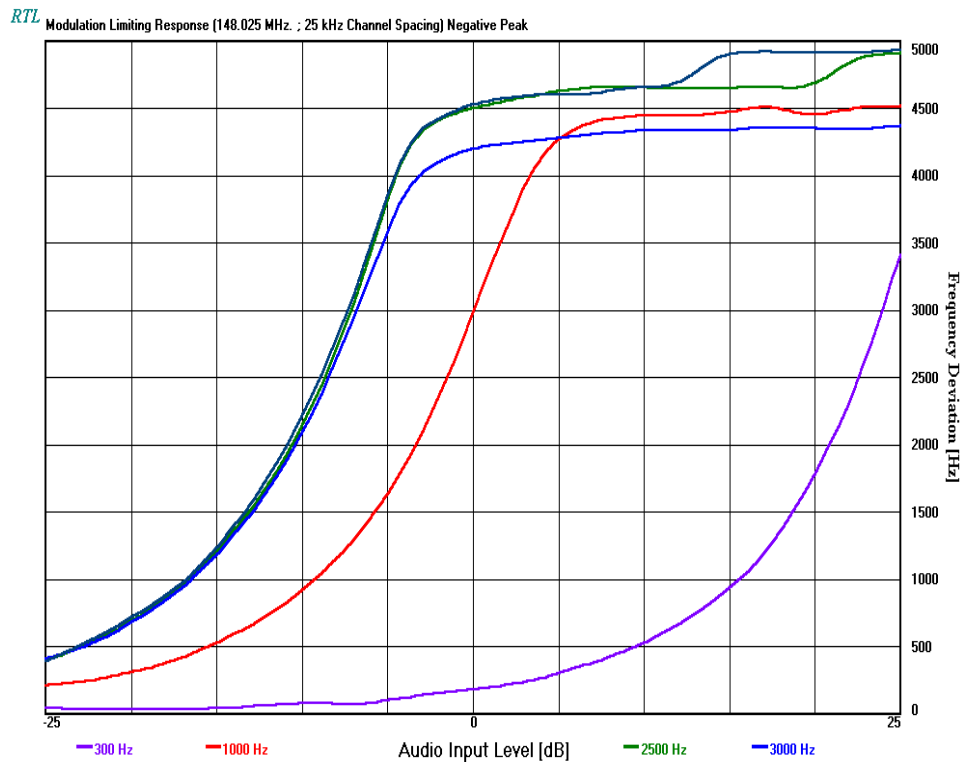
PLOT 13-1: MODULATION CHARACTERISTICS – MODULATION LIMITING: WIDE BAND NEGATIVE PEAK
