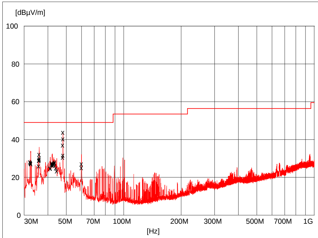
Figure 5.13.1 Radiated Emissions Results Chamber result @ 3m (RE08)
