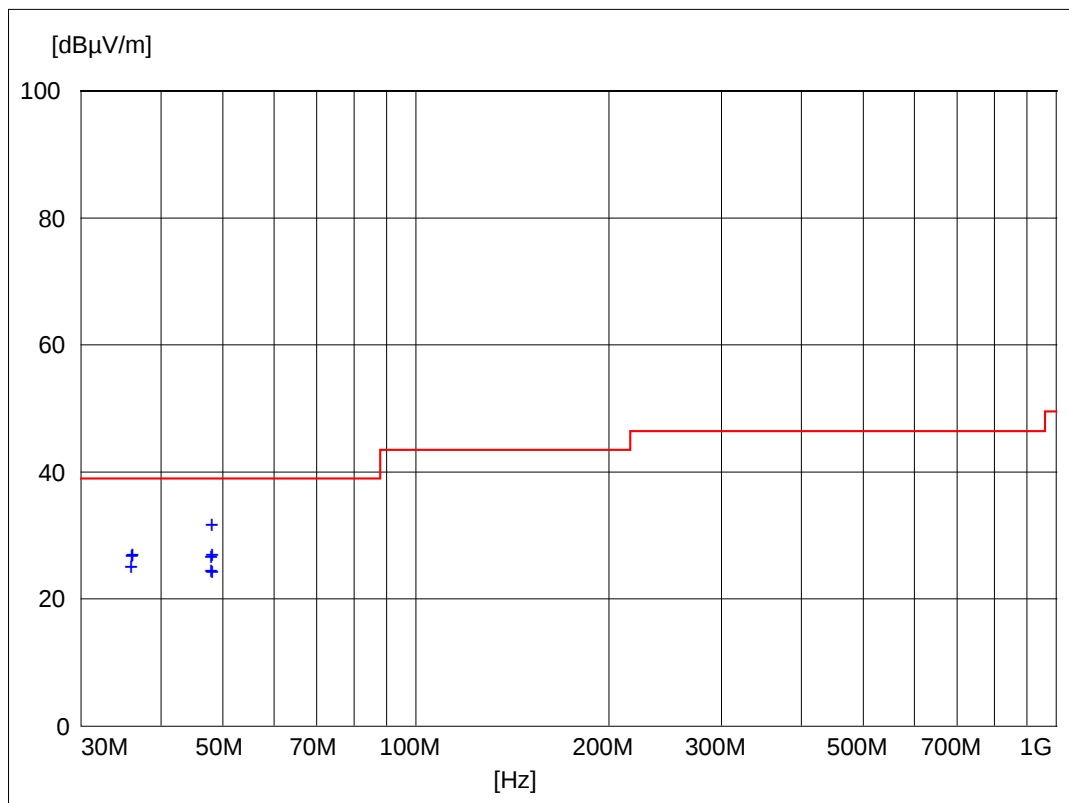
Figure 5.13.2 Radiated Emissions Results Open area test site @10m (RE09)
