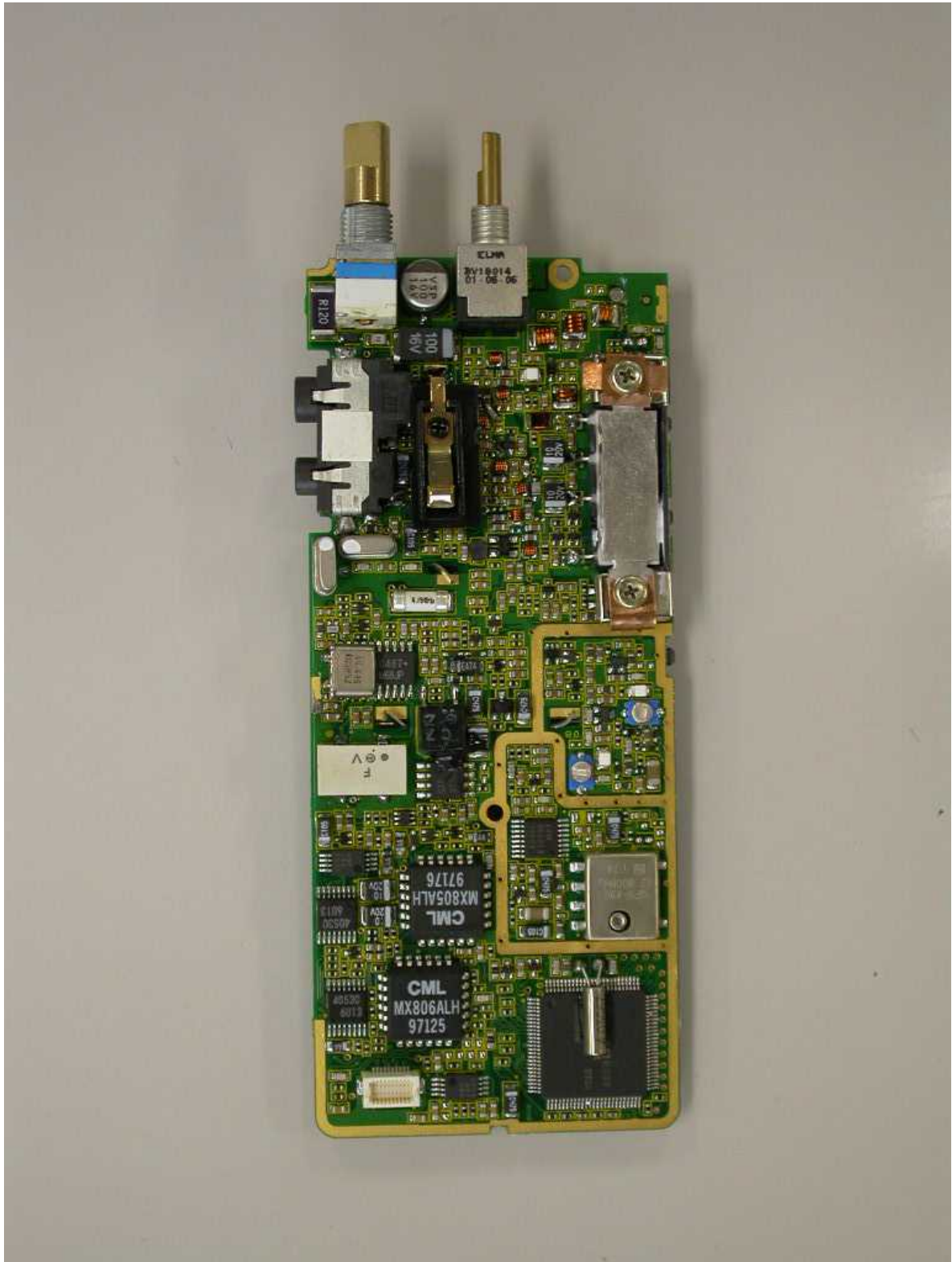
10) MAIN PCB of SC-581 C (Solder Side View)
