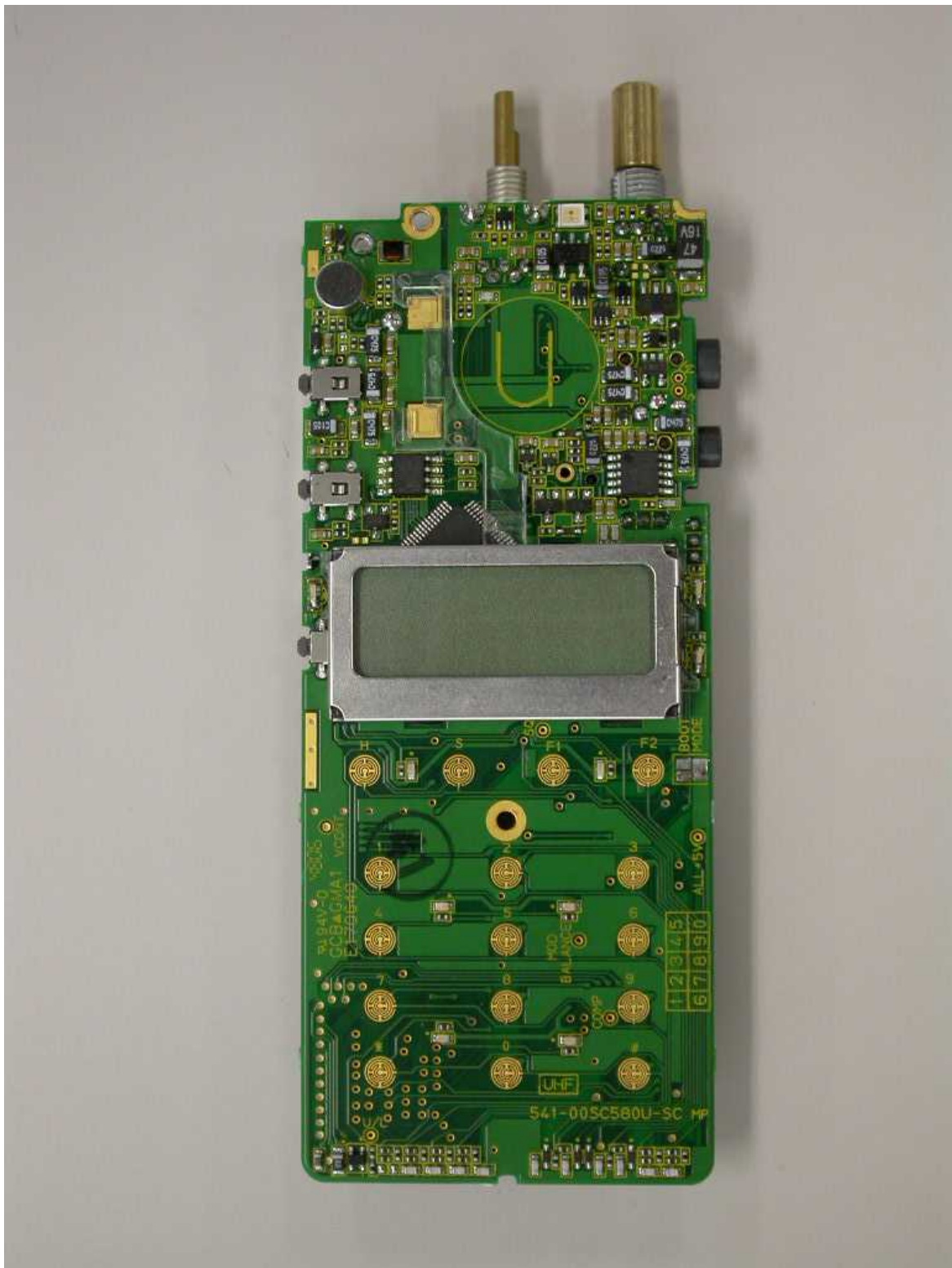
9) MAIN PCB of SC-581 C (Component Side View)
