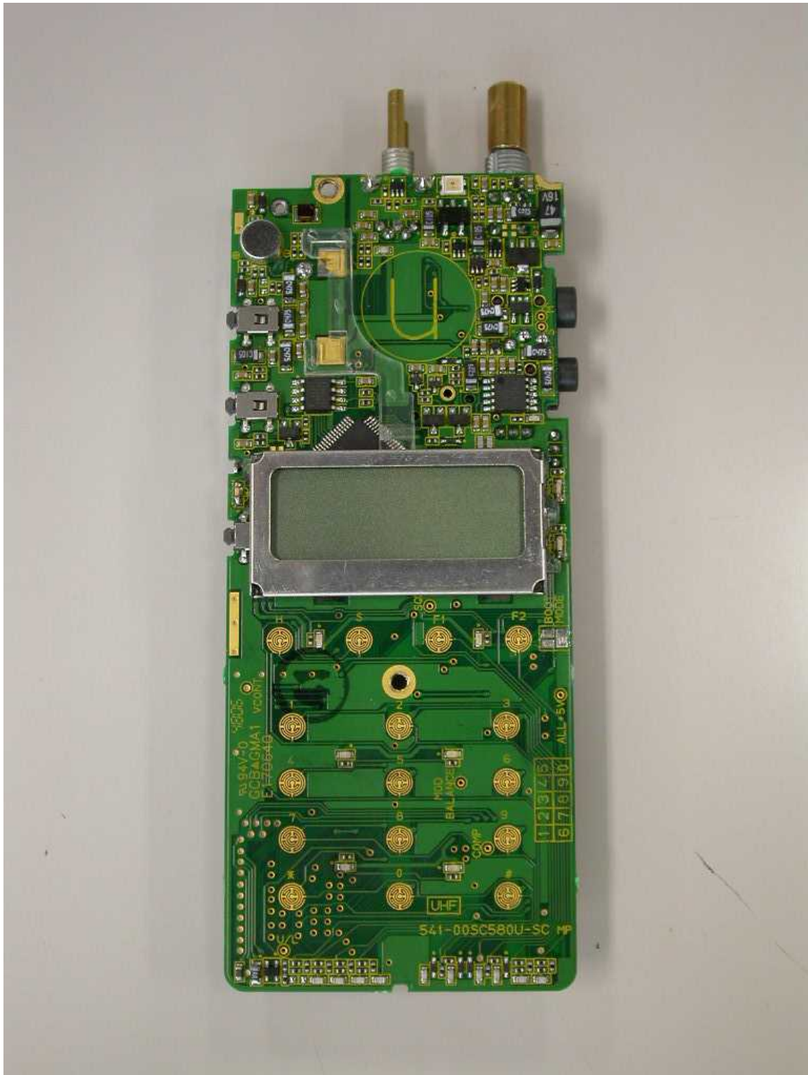
9) MAIN PCB of SC-580 A (Component Side View)
