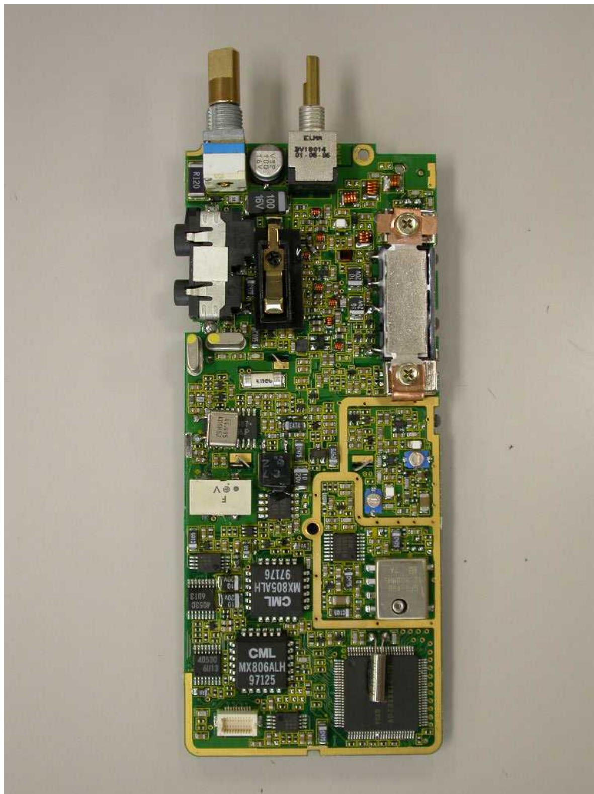
10) MAIN PCB of SC-580 A (Solder Side View)
