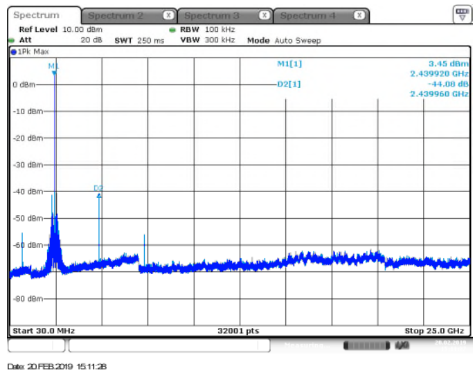
Figure 7.5.1.2-2: MCH – 30MHz–25GHz
