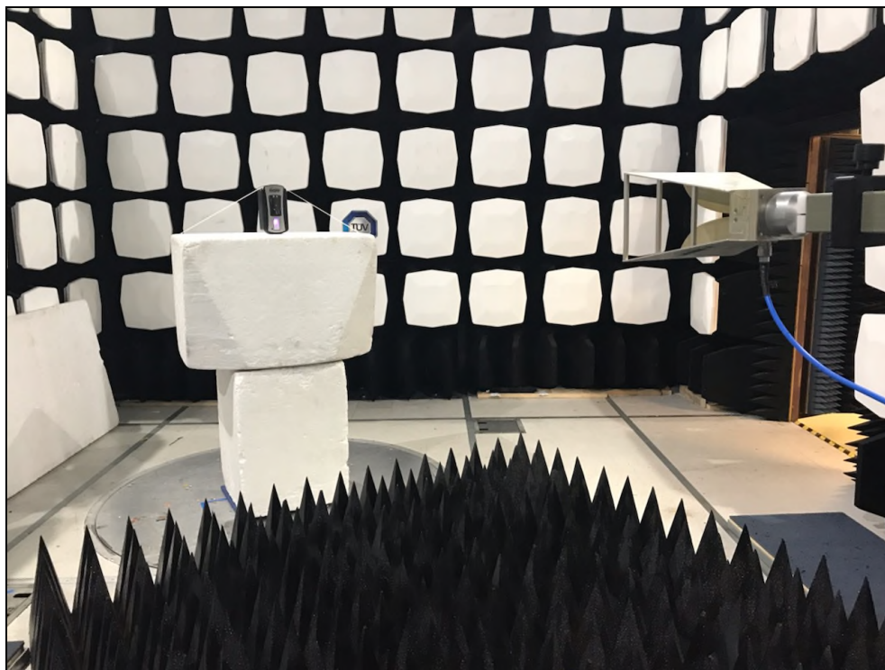
Figure 1: Radiated Emissions Test Setup – LTX Model – Front
