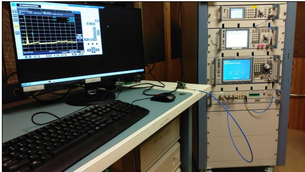
Figure 5: Antenna Port Conducted Test Setup
