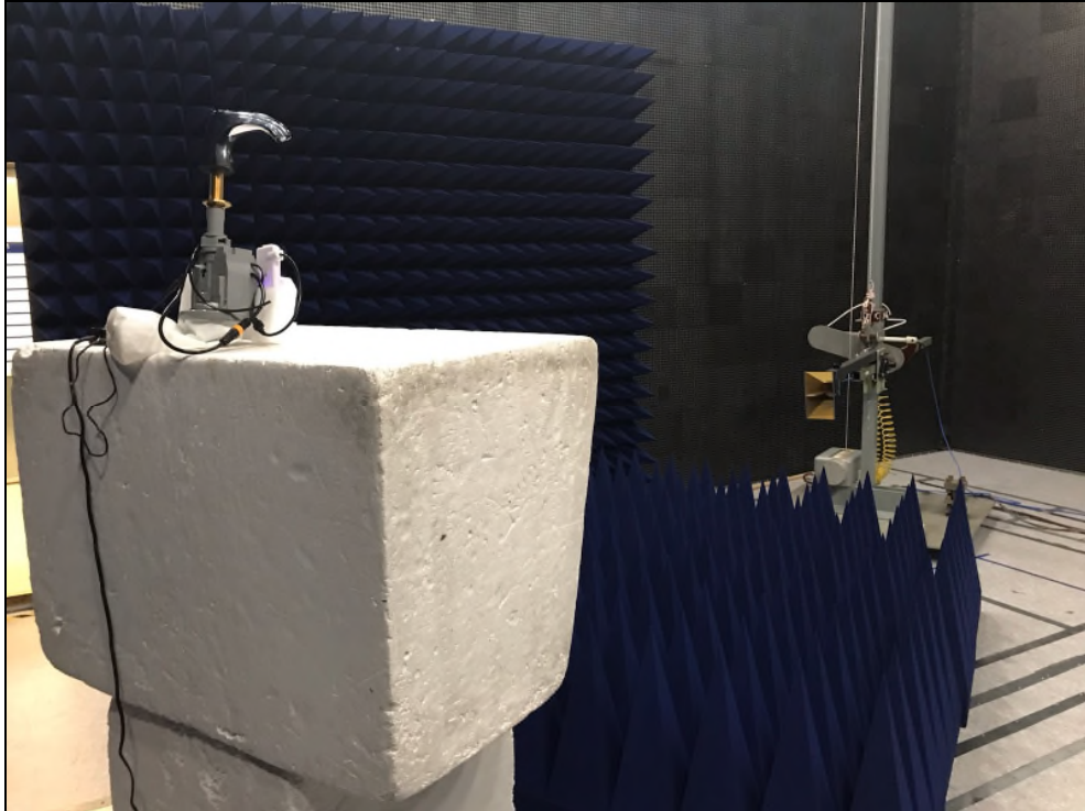
Figure 4: Radiated Emissions Test Setup – CXR Model – Rear
