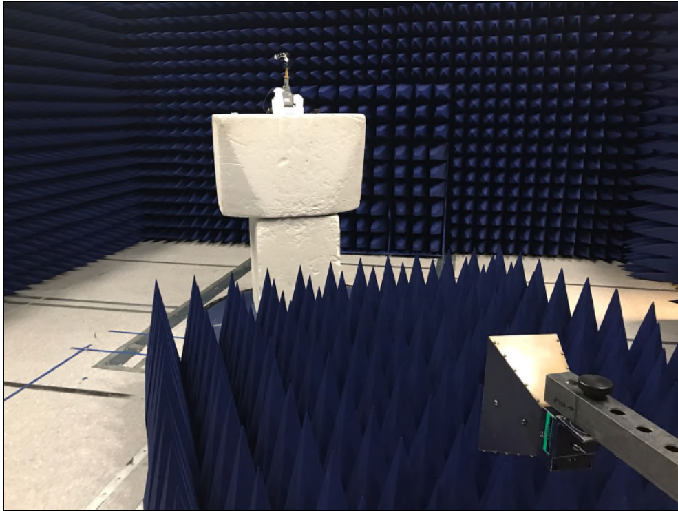
Figure 3: Radiated Emissions Test Setup – CXR Model – Front
