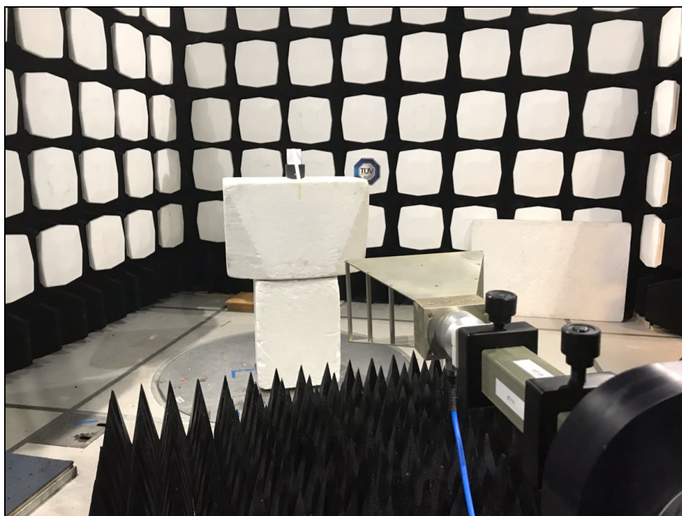
Figure 2: Radiated Emissions Test Setup – ES8 Model – Front
