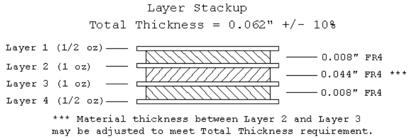
(a) Total Thickness 0.062"
