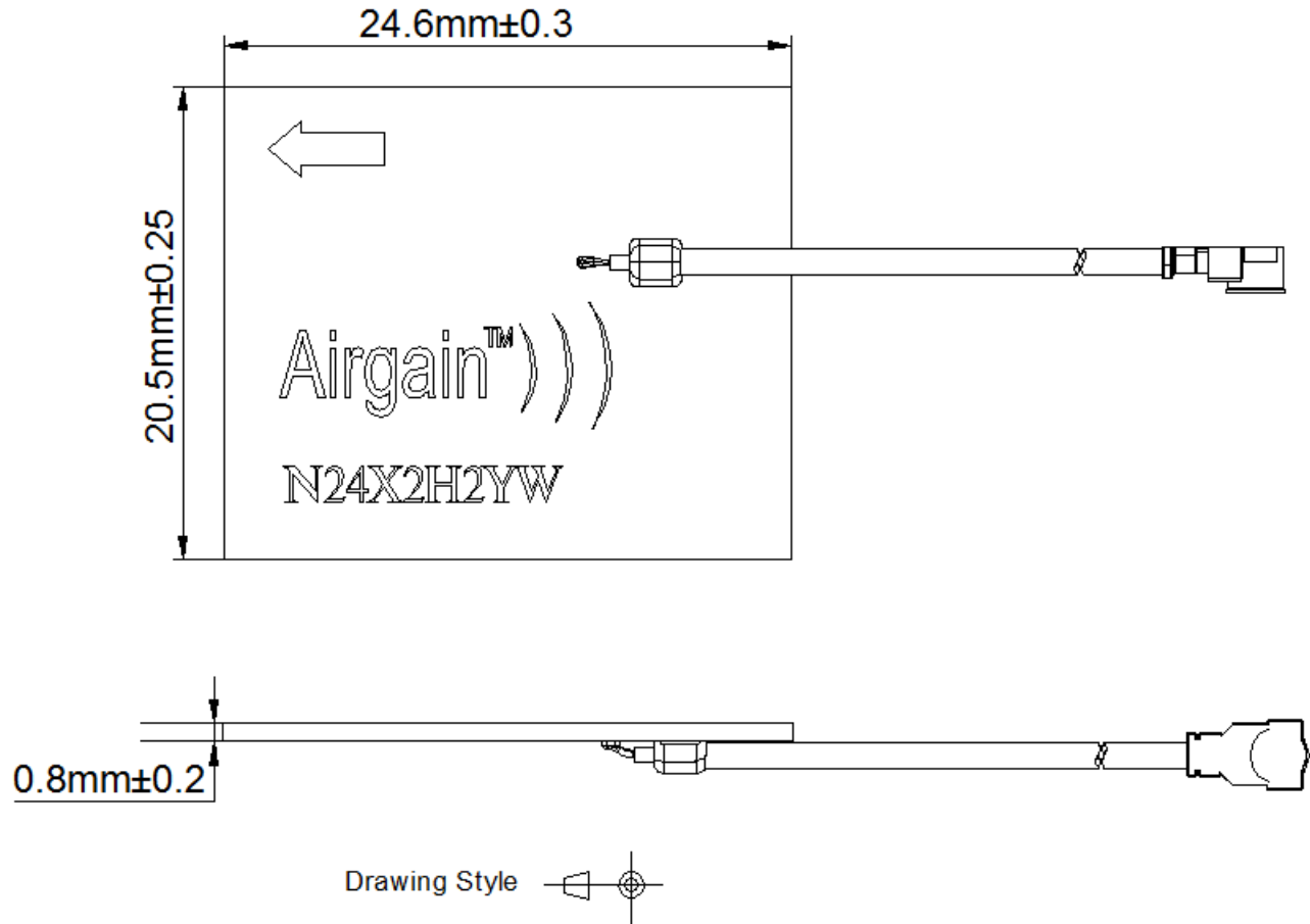
Figure 6: Model N24X2H2YW Embedded Antenna Dimensions
