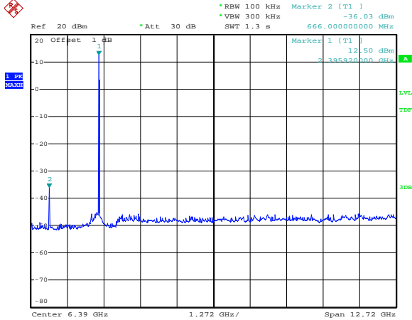
Figure 6. Plot of the Spurious RF conducted emissions Ant0_2.4 GHz 802.11b
