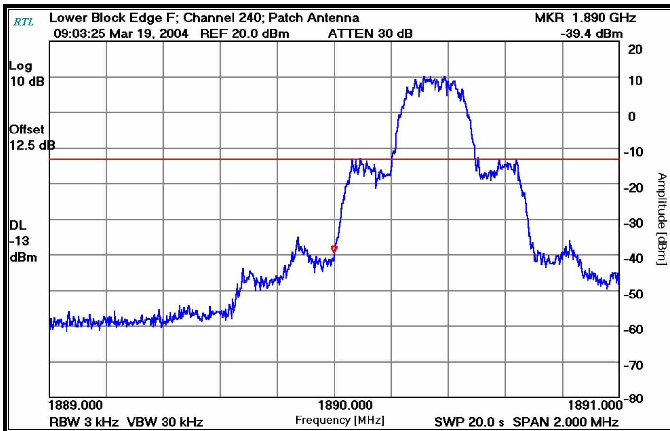
PLOT 8-9: LOWER BAND EDGE BLOCK F - PATCH ANTENNA
