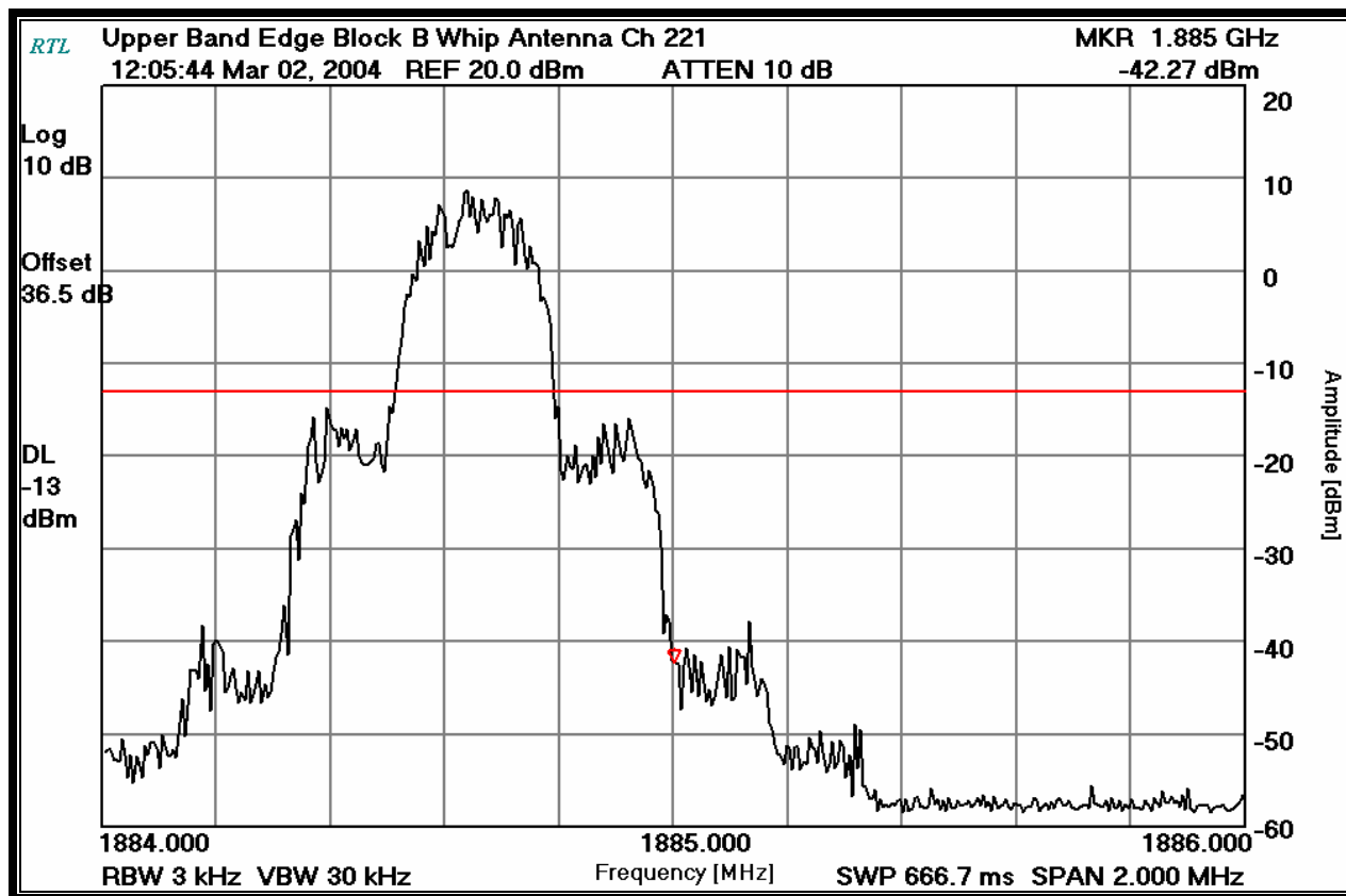
PLOT 8-2: UPPER BAND EDGE BLOCK B - WHIP ANTENNA
