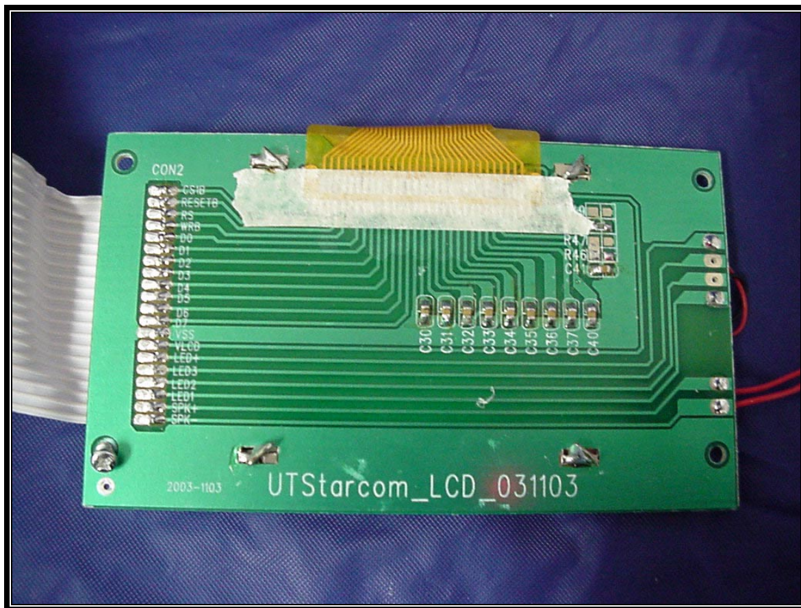
PHOTOGRAPH 37: BOTTOM OF LCD DISPLAY PCB
