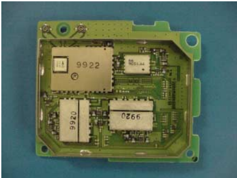
COMPONENT SIDE OF RF PCB
