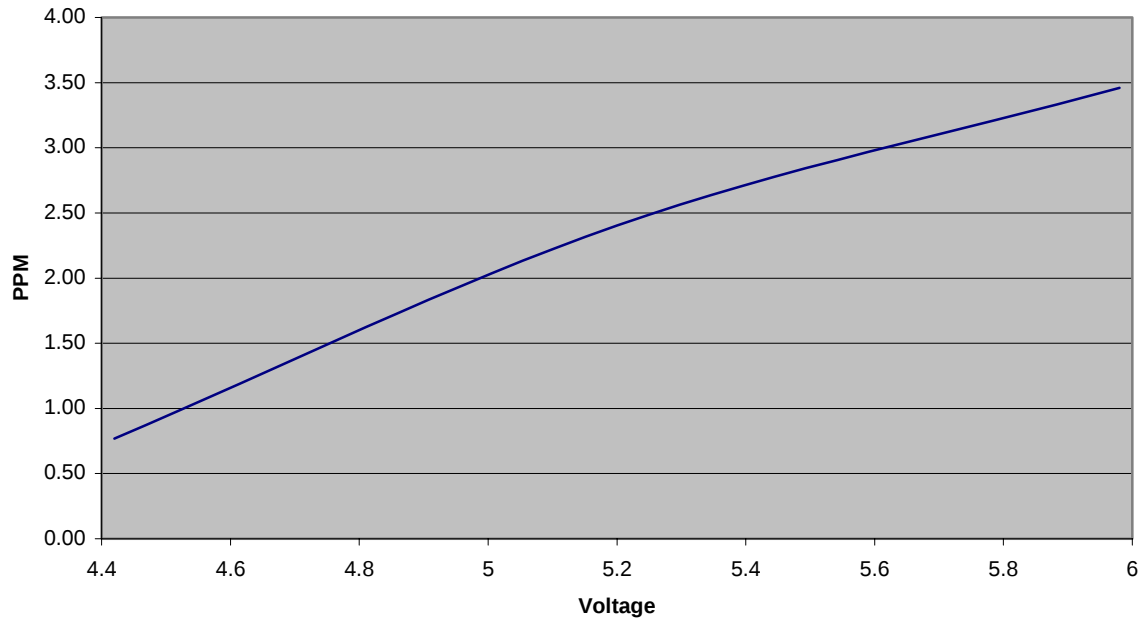
RP Voltage Frequency Stability Nominal Voltage 5.2V
