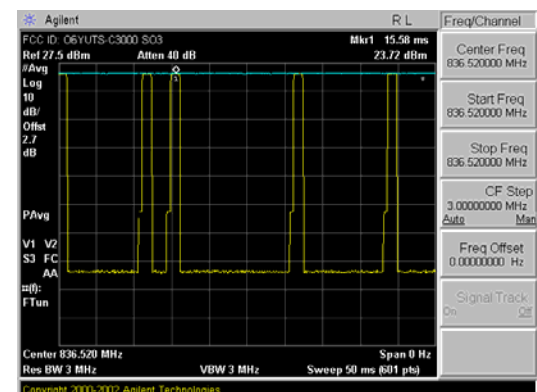
Figure 26 Zero-Span Plots
